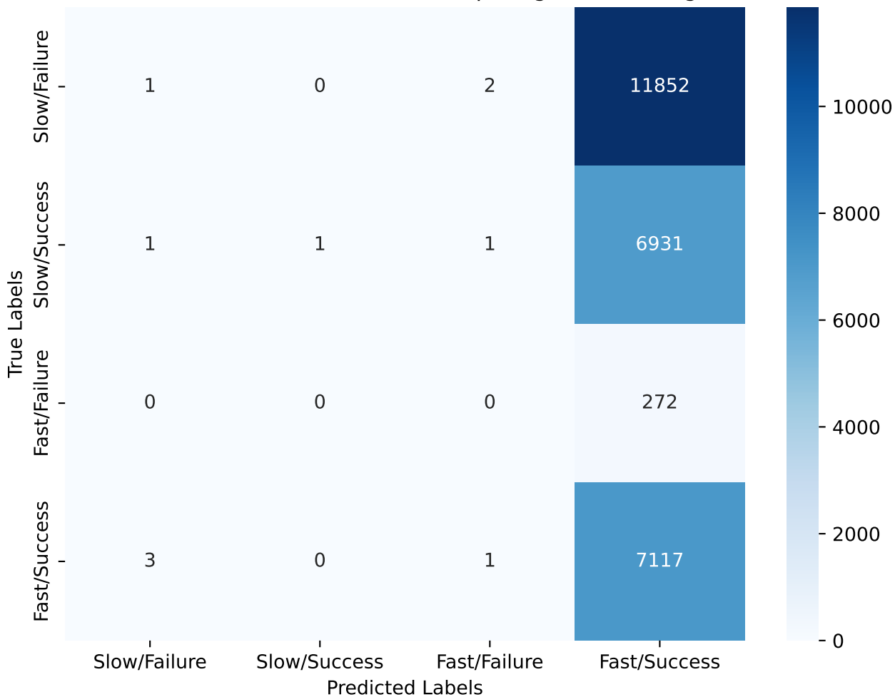
Confusion Matrix for 2-level GraphSage embedding
