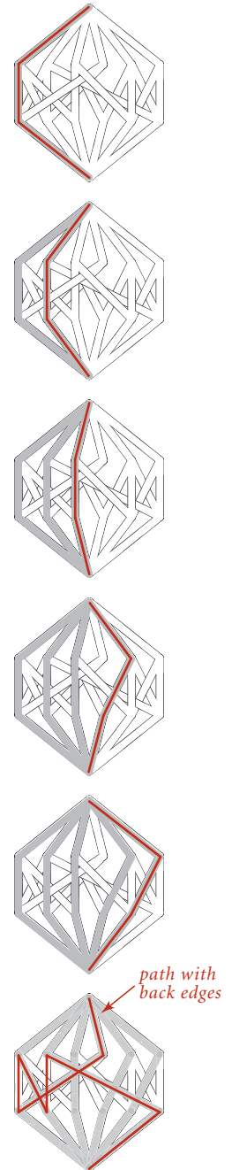
Augmenting paths for bipartite matching
