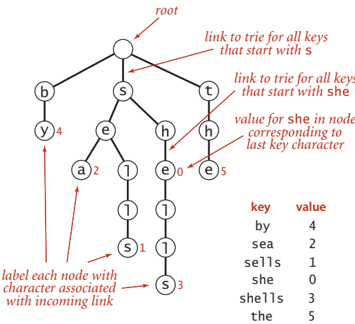
Anatomy of a trie
