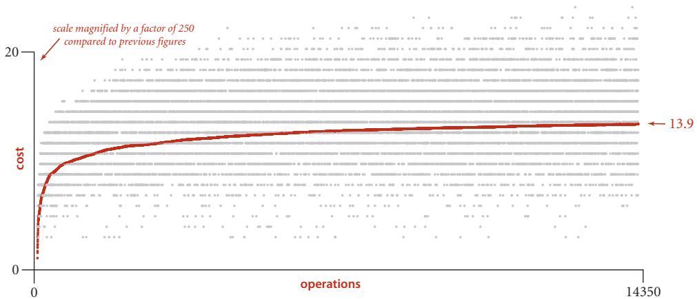
Costs for java FrequencyCounter 8 &lt; tale.txt using BST
