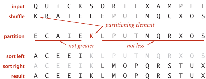
Quicksort overview
