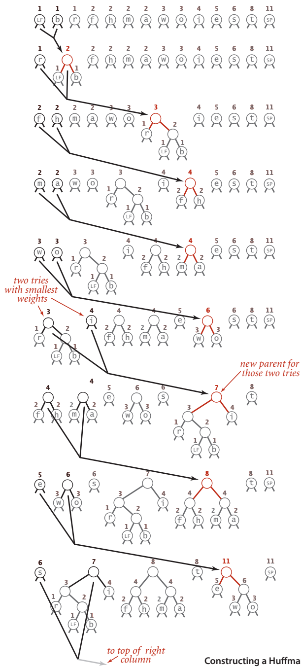
Constructing a Huffman encoding trie
