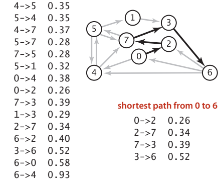
An edge-weighted digraph and a shortest path
