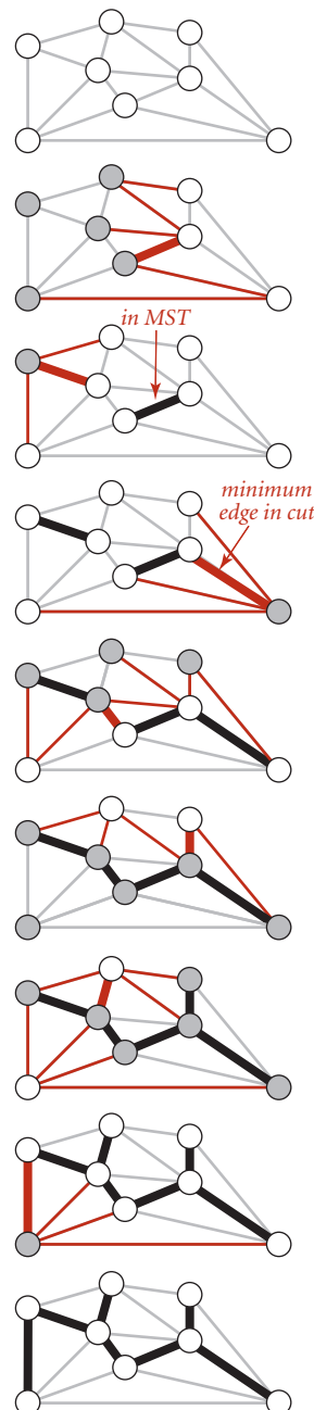
Greedy MST algorithm
