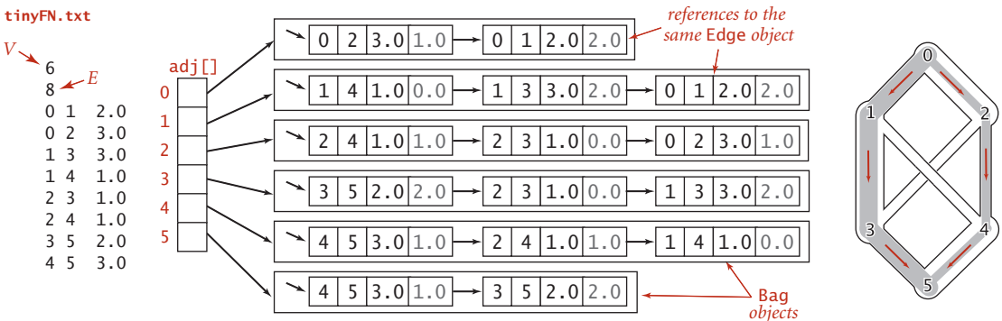
Flow network representation
