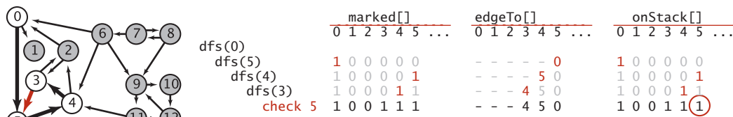
Finding a directed cycle in a digraph
