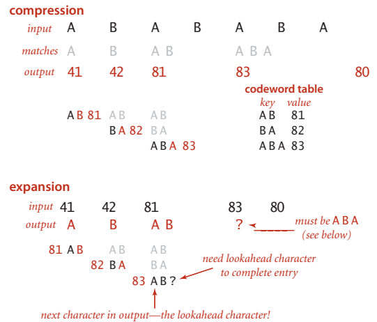
LZW expansion: tricky situation
