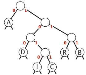
A Huffman code
