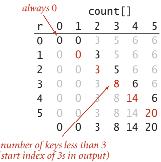
Transforming counts to start indices
