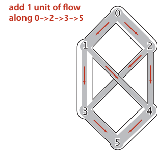
Adding flow to a network
