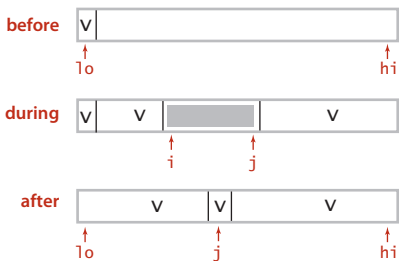
Quicksort partitioning overview
