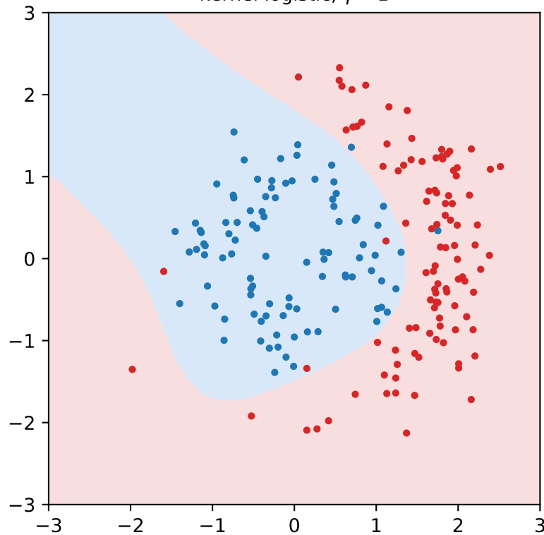
kernel logistic, \gamma = 1
