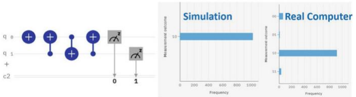
Figure 2 The quantum circuit in Fig. 1 built in IBM-Q. The simulation result is shown in the middle, and the real quantum computer execution result is shown on the right.
