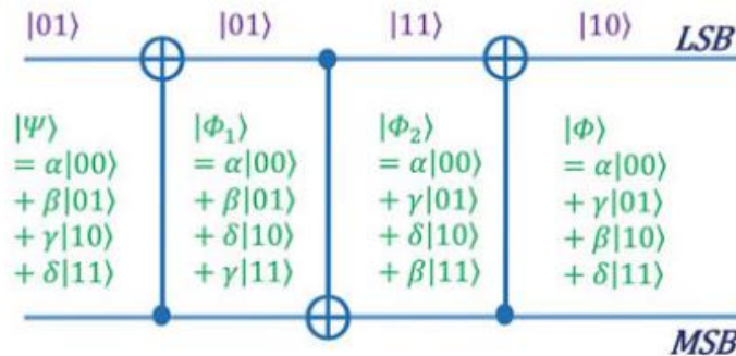
Figure 1 Implementation of a SWAP gate using CNOT gates. The purple ket's on top shows an example of how a single basis vector evolves in the circuit.
