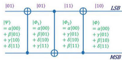
Figure 1 Implementation of a SWAP gate using CNOT gates. The purple ket's on top shows an example of how a single basis vector evolves in the circuit.
