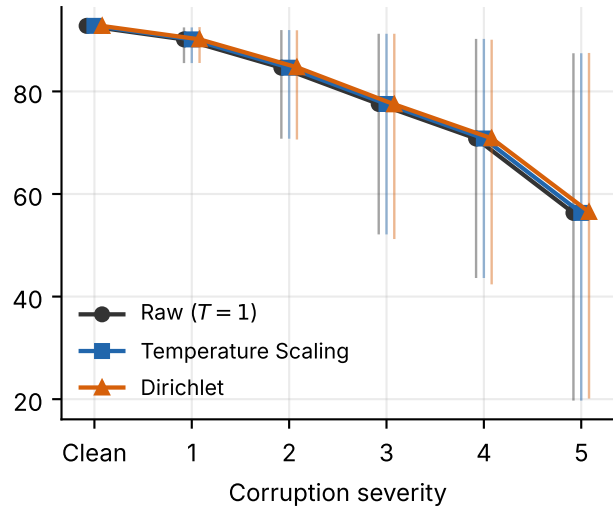
Accuracy (%)
