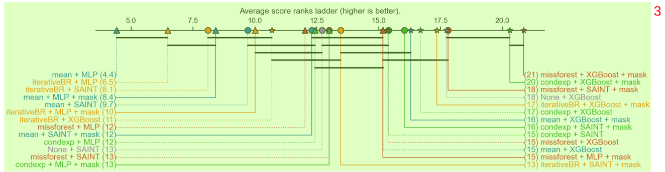
Figure 7: Critical Difference diagram - 50% missingness rate. 4
