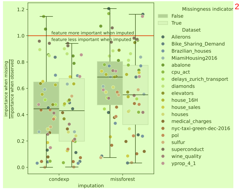
Figure 13: Ratio of importances (when missing over when observed) for the two most important features of each dataset. Importances are calculated with feature permutation. The 2 most important features per dataset are identified based on the whole test set. For each feature j , a permutation importance is then calculated based on the subset of test samples where feature j is missing, and the subset where it is observed. The ratio between these two values is then reported on the figure, where a point refers to one feature, and its color identifies the dataset it belongs to. A ratio of 1 indicates that the feature is as important whether it is imputed or observed (red line). A ratio of 0.1 means that it is 10 times less important when it is imputed compared to when it is observed. 3
