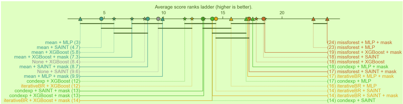
Figure 8: Critical Difference diagram - 20% missingness rate, semi-synthetic data with linear outcomes. 6
