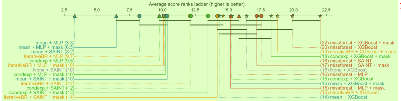
Figure 6: Critical Difference diagram - 20% missingness rate. 2
