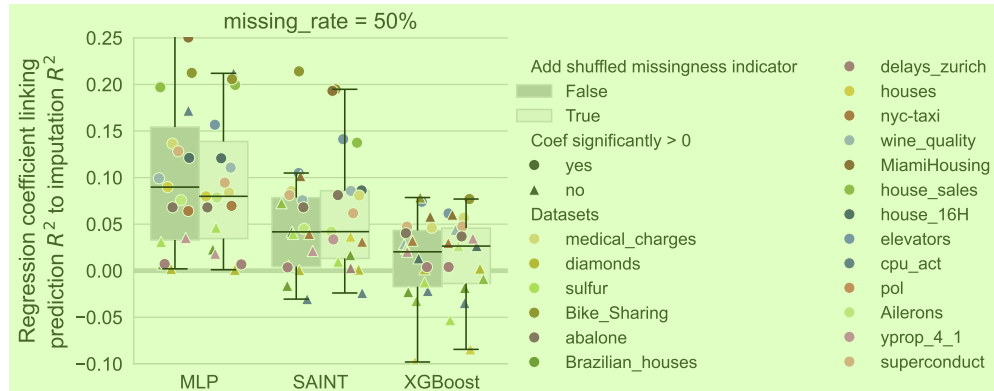
(a) Effect of appending a shuffled mask on prediction performances. Real outcome, 50% MCAR missingness. 3
