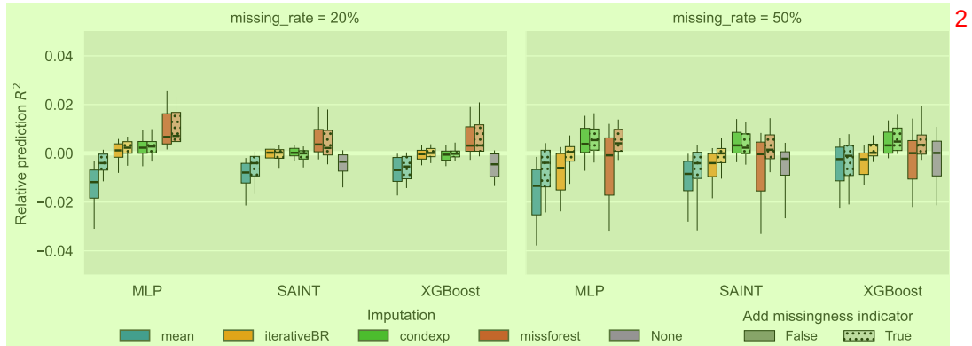
Figure 10: Relative prediction performances for the semi-synthetic data with linear outcomes across datasets for different imputations, predictors, and use of the missingness indicator. Each boxplot represents 200 points (20 datasets with 10 repetitions per dataset). The performances shown are R^2 scores on the test set relative to the mean performance across all models for a given dataset and repetition. A value of 0.01 indicates that a given method outperforms the average performance on a given dataset by 0.01 on the R^2 score. 3
