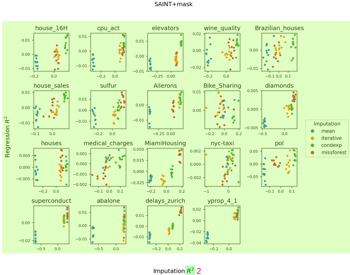
Figure 27: Prediction R^2 vs imputation R^2 for SAINT + indicator semi-synthetic data with linear outcomes, missing rate 50%. The R^2 scores are given relative to the mean R^2 score, with the effects of experiment repetitions eliminated (i.e. the effect of the train/test splits on the performance)
