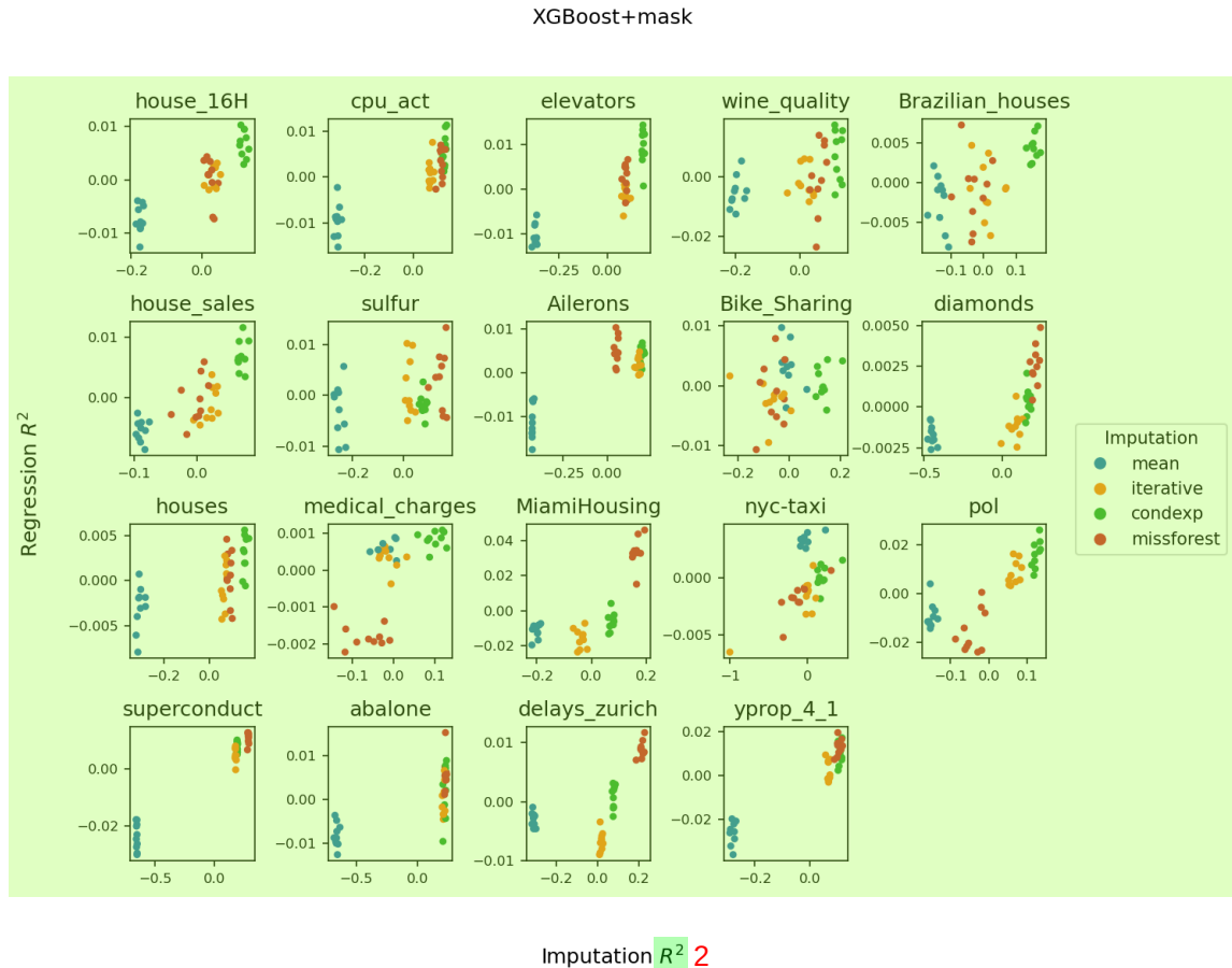
Figure 29: Prediction R^2 vs imputation R^2 for XGBoost + indicator semi-synthetic data with linear outcomes, missing rate 50%. The R^2 scores are given relative to the mean R^2 score, with the effects of experiment repetitions eliminated (i.e. the effect of the train/test splits on the performance)
