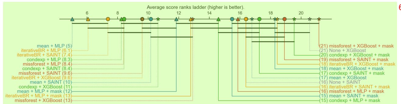
Figure 32: Critical Difference diagram - 50% missingness rate under MNAR missingness. 7
