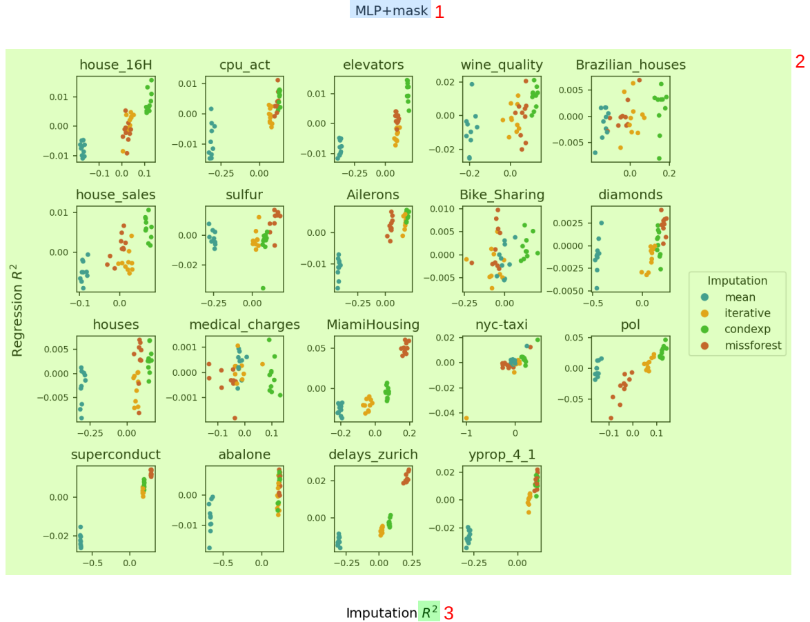
Figure 25: Prediction R^2 vs imputation R^2 for a MLP + indicator - 4 semi-synthetic data with linear outcomes, missing rate 50%. The R^2 scores are given relative to the mean R^2 score, with the effects of experiment repetitions eliminated (i.e. the effect of the train/test splits on the performance)
