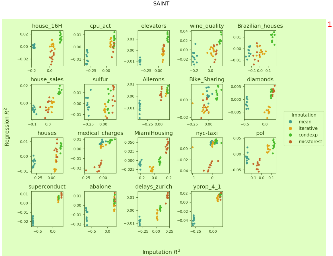
Figure 26: Prediction R^2 vs imputation R^2 for SAINT - semi-synthetic data with linear outcomes, 2 missing rate 50%. The R^2 scores are given relative to the mean R^2 score, with the effects of experiment repetitions eliminated (i.e. the effect of the train/test splits on the performance)
