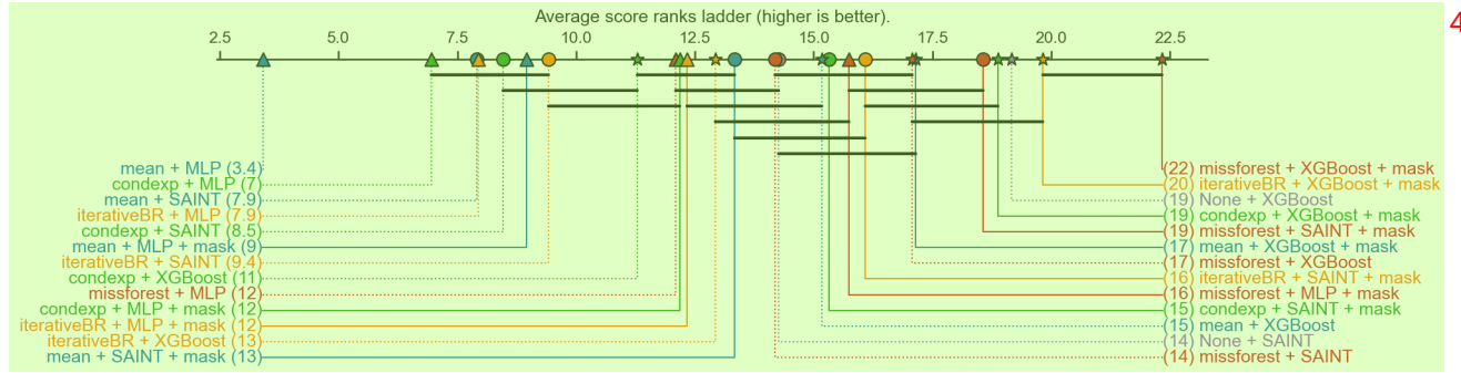
Figure 31: Critical Difference diagram - 20% missingness rate under MNAR missingness. 5
