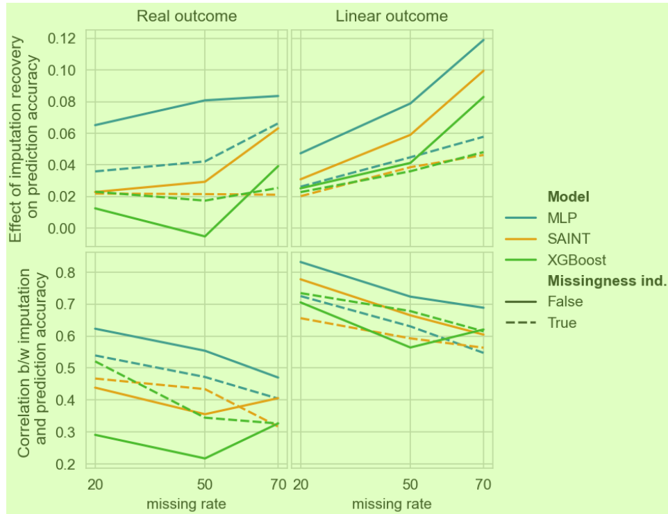
Figure 12: Increasing missing rates lead to larger effects (slopes) but noisier associations (lower correlation). The values reported are median across datasets, for each model. Data is MCAR. 3
