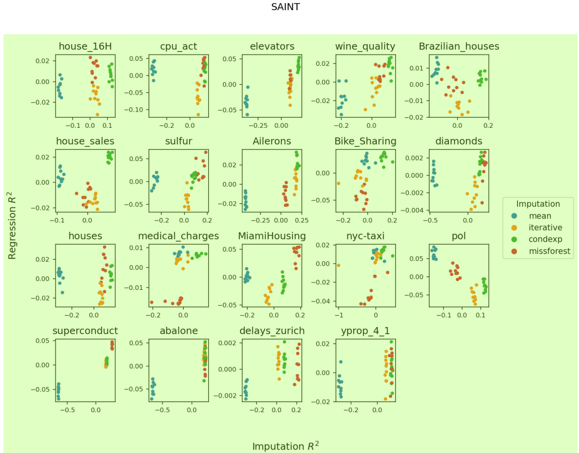
Figure 20: Prediction R^2 vs imputation R^2 for SAINT - missing rate 50%. The R^2 scores are given 2 relative to the mean R^2 score, with the effects of experiment repetitions eliminated (i.e. the effect of the train/test splits on the performance)
