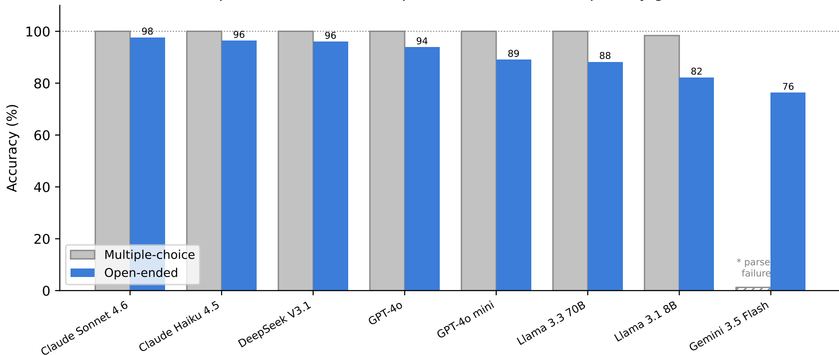
Multiple-choice saturates; open-ended reveals a capability gradient
