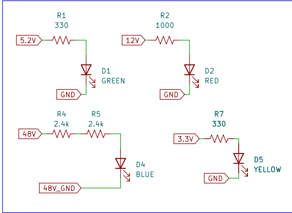
Voltage LEDs
