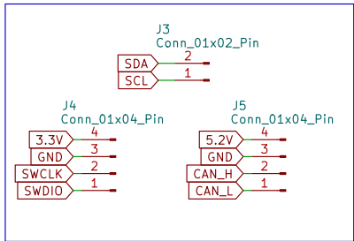
Debugging Pins
