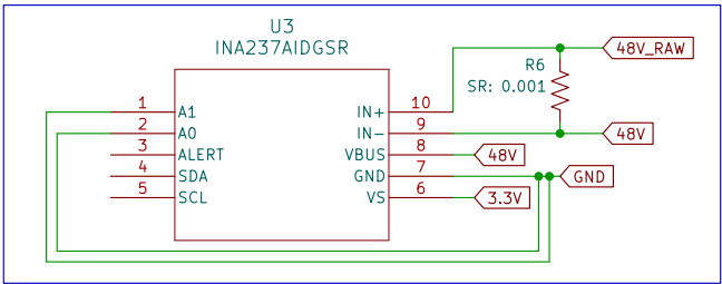
Power Monitor IC
