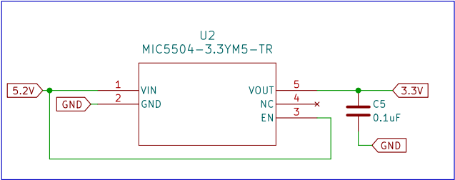
3.3V LDO
