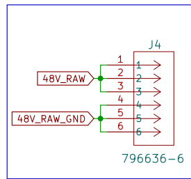
Tether Wall Connector
