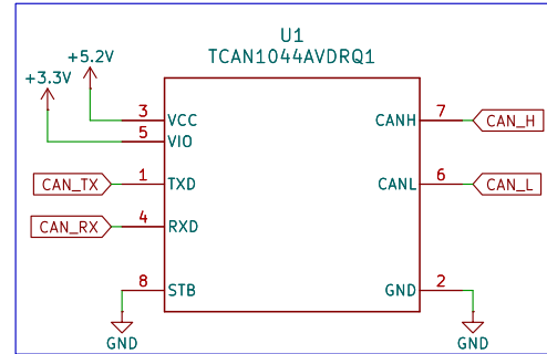
CAN Transceiver
