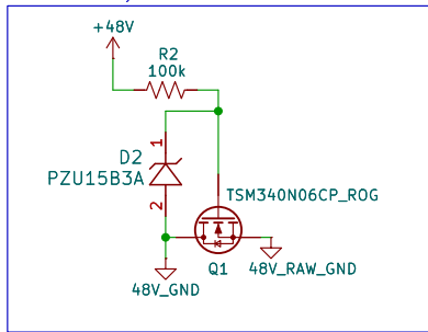
Reverse Polarity Protection
