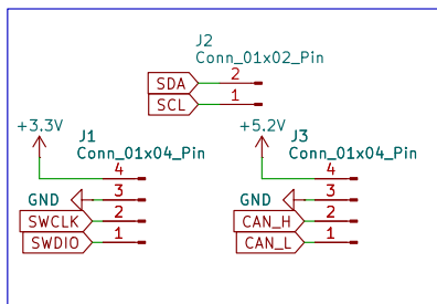
Debugging Pins
