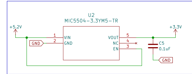
3.3V LDO
