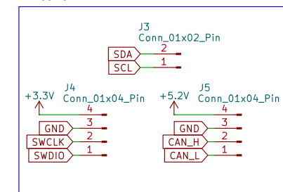
Debugging Pins
