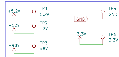
Test Points
