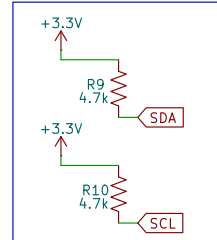
I2C
