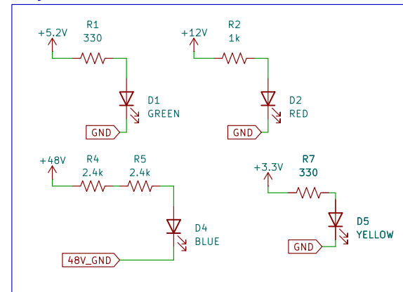
Voltage LEDs
