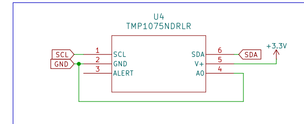
Temp Sensor
