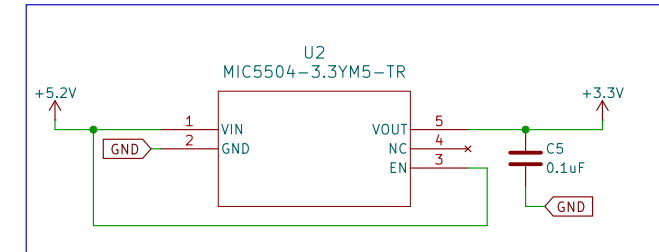
3.3V LDO
