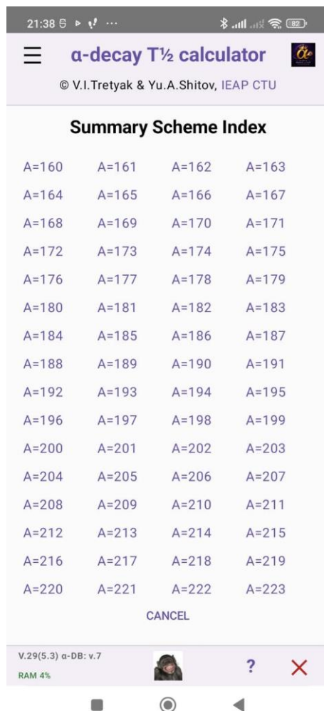
Figure 7. Mass-number index A.
