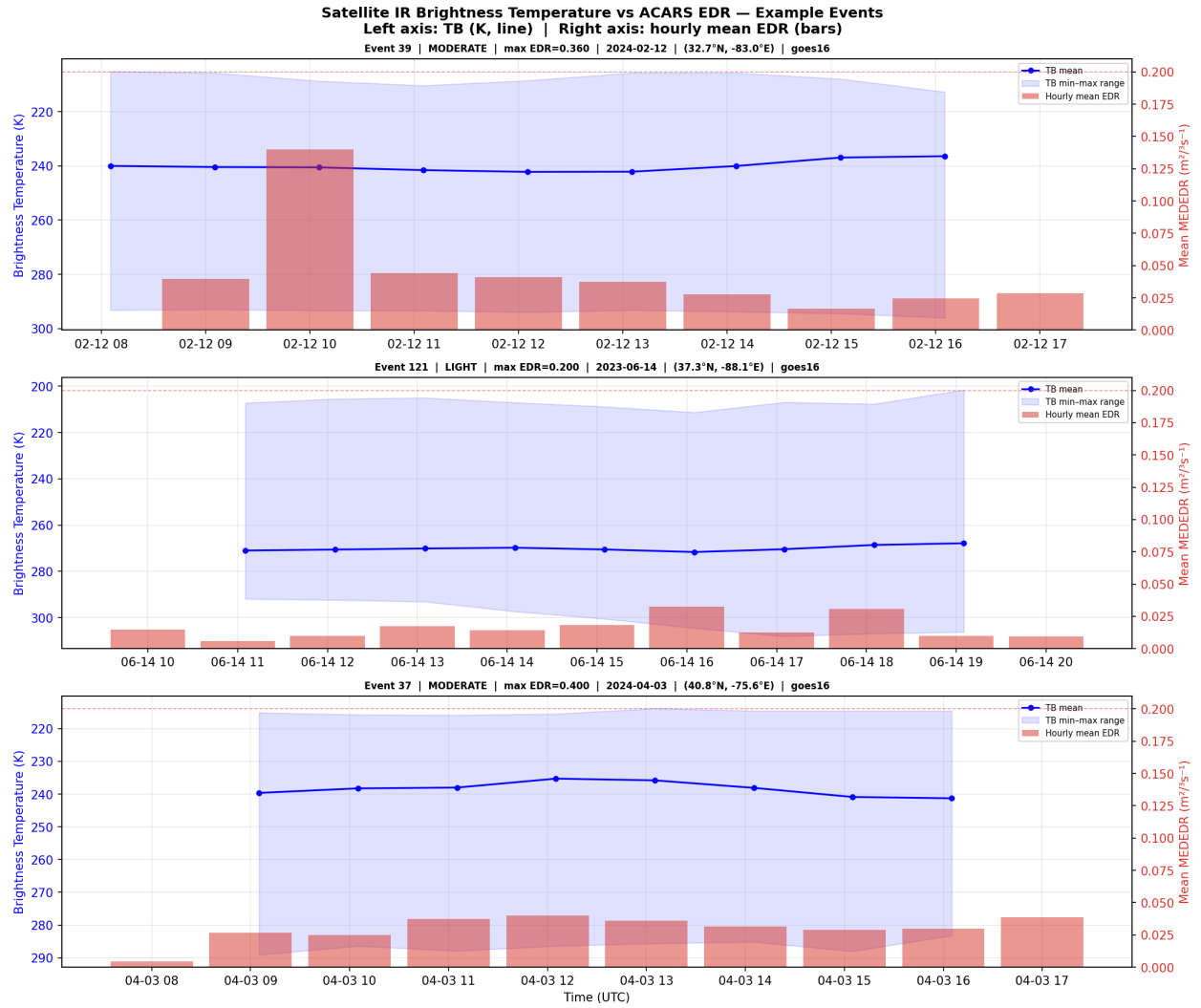
Figure 11: Example events: satellite IR brightness temperature (line) vs. hourly mean EDR (bars). Cloud-top cooling tends to lead EDR peaks in convective cases.
