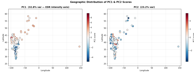
Figure 14: Geographic distribution of PC1 (EDR-intensity) and PC2 scores by event centroid; most intense events cluster at higher latitudes.
