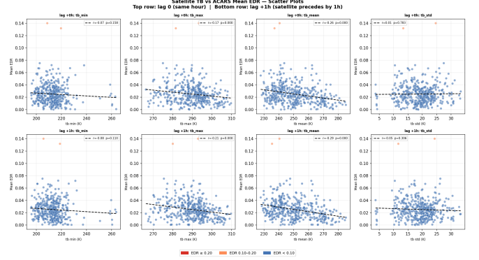
Figure 10: Satellite TB vs. ACARS mean EDR scatter at lag 0 (top) and lag +1 h (bottom). Colder tb_mean/tb_max associates with higher EDR; severe clear-sky events (no cold cloud) are the off-trend outliers.
