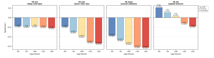
Figure 9: Spearman correlation of satellite brightness-temperature statistics with ACARS mean EDR at lags -2 to +2 h. Positive lag = satellite precedes turbulence; tb_mean at +2 h gives r = -0.31 .
