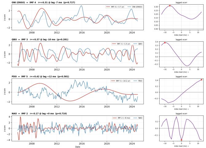
Figure 6: Lagged cross-correlations of EEMD turbulence modes against climate indices (ONI, QBO, PDO, NAO). All correlations are non-significant under 1000 phase-randomised surrogates ( p > 0.05 ).
