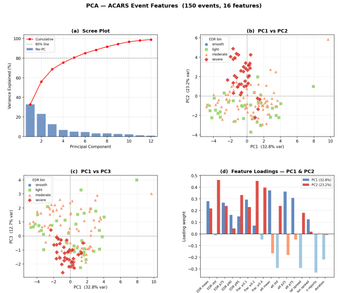
Figure 12: PCA of ACARS event features (150 events, 16 features). PC1 (32.8%) is an EDR-intensity axis along which severe events separate; scree, PC1-PC2, PC1-PC3, and feature loadings shown.
