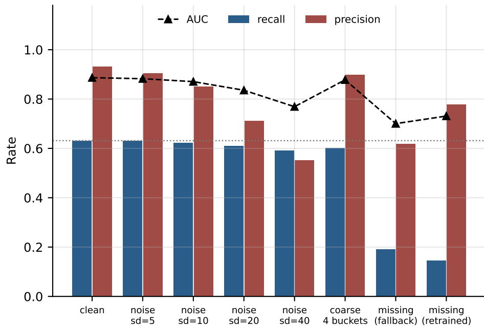
(a) At the fixed 0.5 threshold, as submitted alert rate is free to move (19% \rightarrow 30% under noise)
