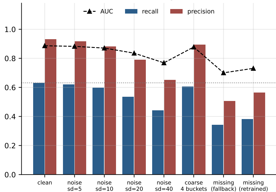
(b) At a matched alarm budget (19.0% alerts) noise now costs recall too; missing information most of all
