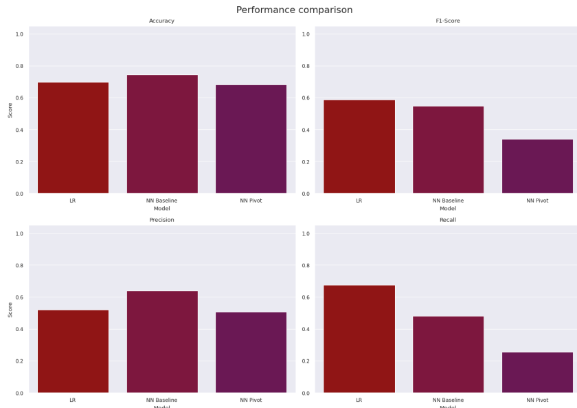
Figure 2: Graphical performance comparison across accuracy, precision, recall, and F1-score.
