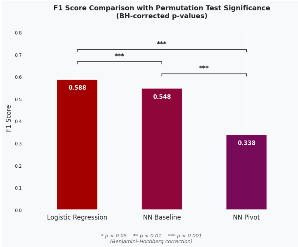
Figure 3: Pairwise comparison of F1 scores using permutation testing with Benjamini–Hochberg correction. All pairwise differences are significant at p < 0.001 .
