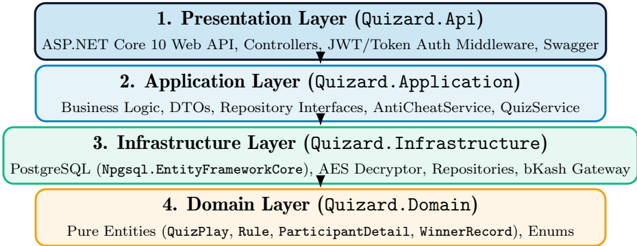
Figure 16.1: Quizard .NET 10 Clean Architecture Dependency Hierarchy
