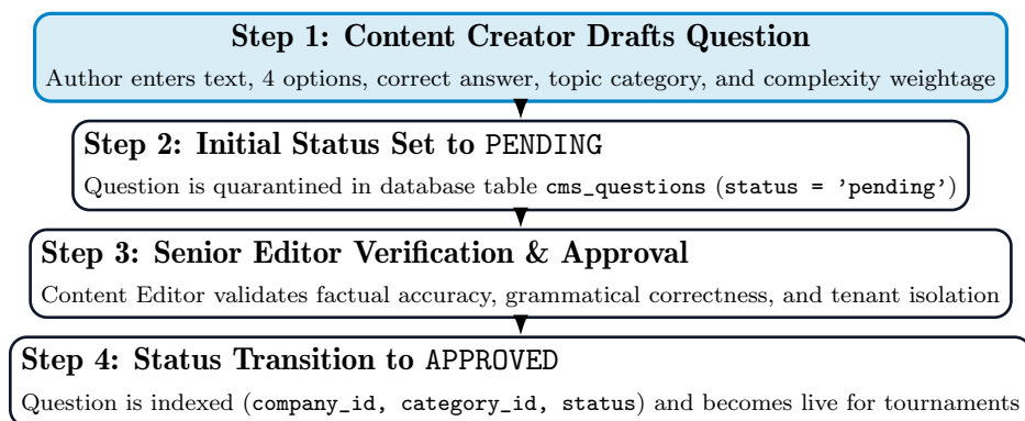
Figure 10.1: The Multi-Stage CMS Question Approval Pipeline
