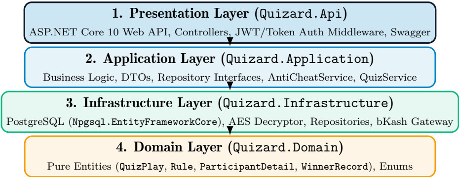
Figure 12.1: Quizard .NET 10 Clean Architecture Dependency Hierarchy
