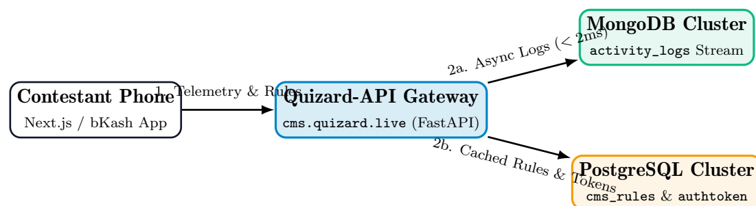
Figure 9.1: Quizard-API ( cms.quizard.live ) Asynchronous Ingestion & Caching Architecture
