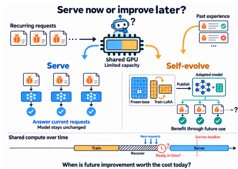
LearnSched preprint Figure 1: a shared GPU trades current service against future improvement and pays a recovery cost [22]
