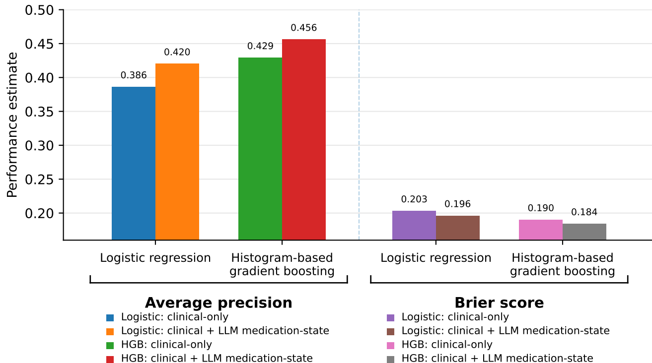
Test-set performance by average precision and Brier score
