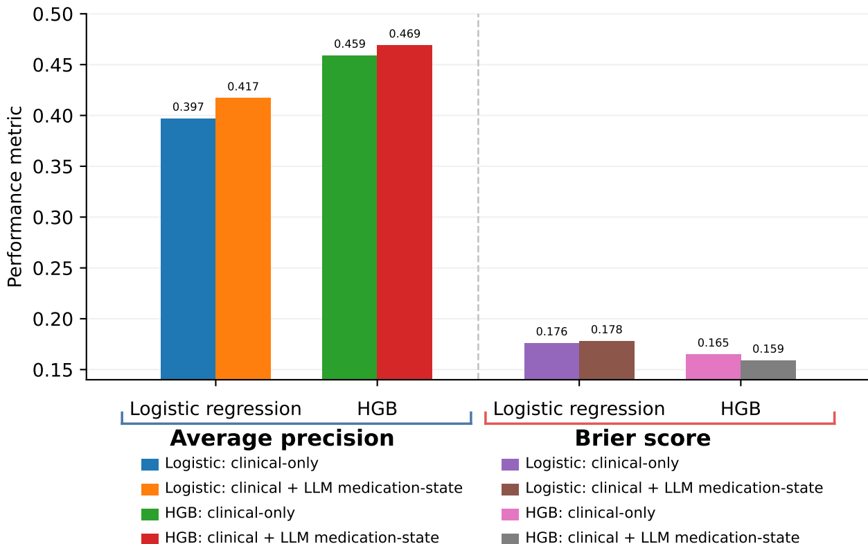
Temporal test-set performance by average precision and Brier score
