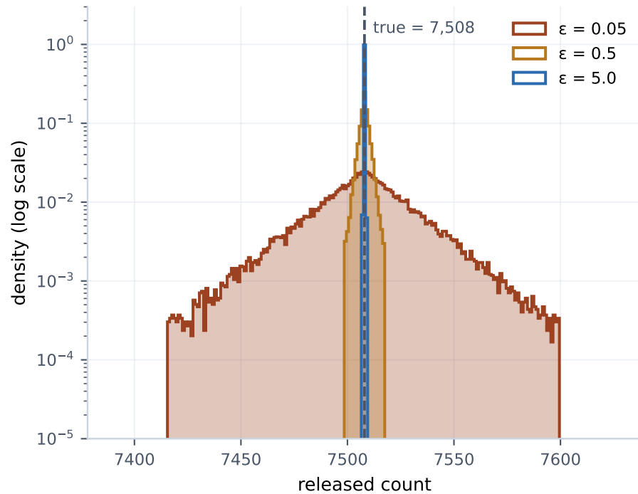
(b) What the released answer actually looks like
