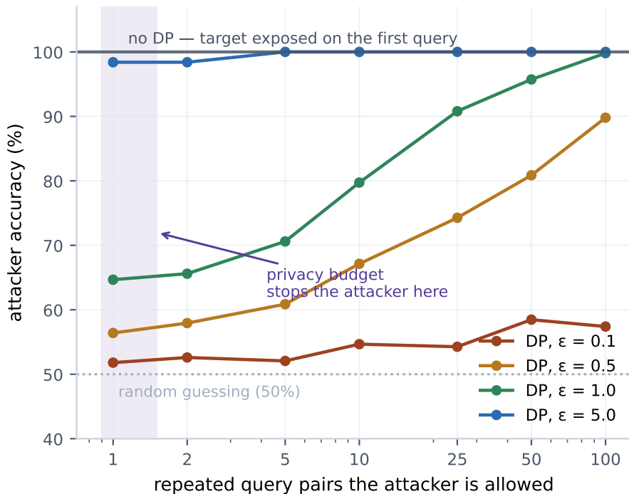
(a) Differencing attack: noise alone is not enough
