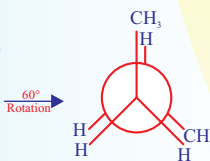
Partially Eclipsed form
