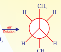
Anti Staggered-form (most stable)
