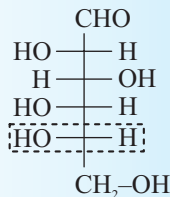
L-Glucose
