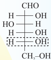
D-Glucose
