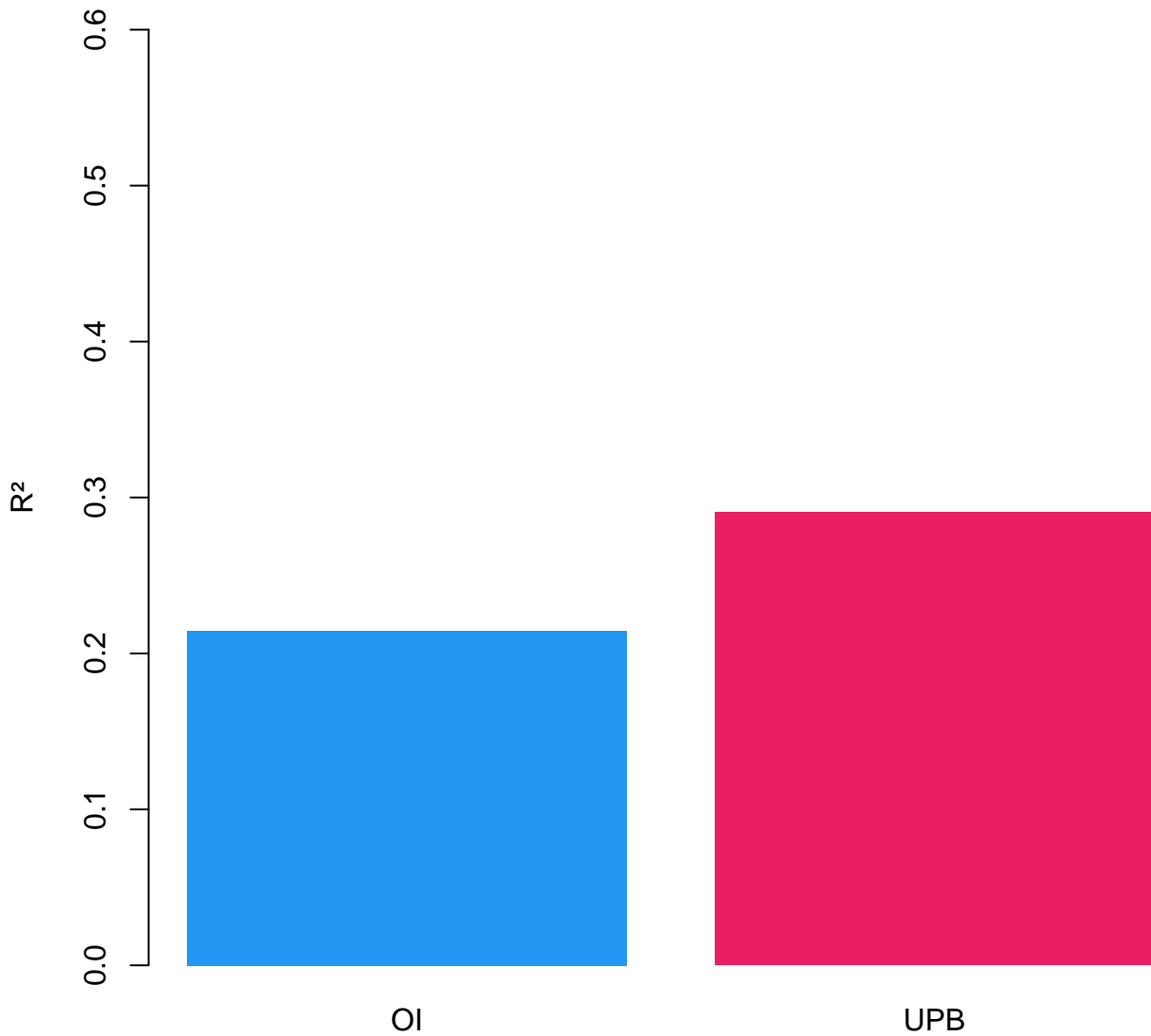
R-squared (Variance Explained)
