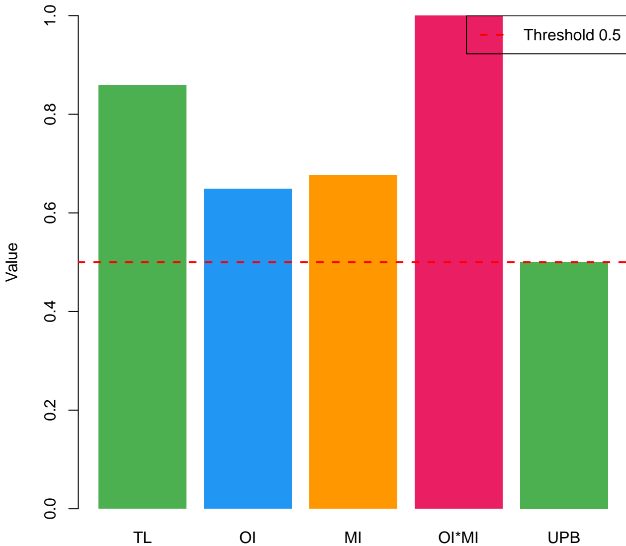
Average Variance Extracted (AVE)
