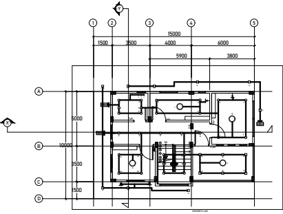
THIRD FLOOR LIGHTING LAYOUT SCALE: 1:150
