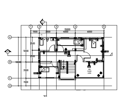
THIRD FLOOR POWER & AUXILIARY LAYOUT SCALE: 1:150
