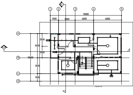
SECOND FLOOR LIGHTING LAYOUT SCALE: 1:150
