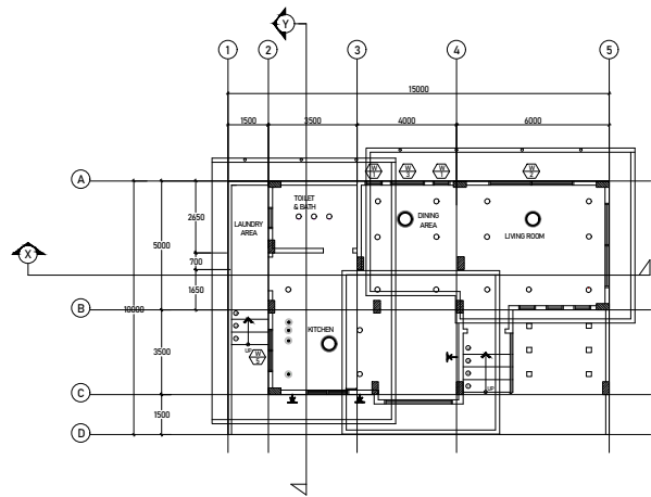
GROUND FLOOR REFLECTED CEILING PLAN SCALE: 1:100
