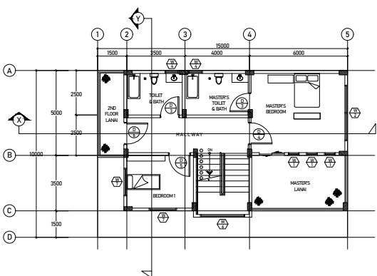
5 A 2 SECOND FLOOR PLAN SCALE: 1:100
