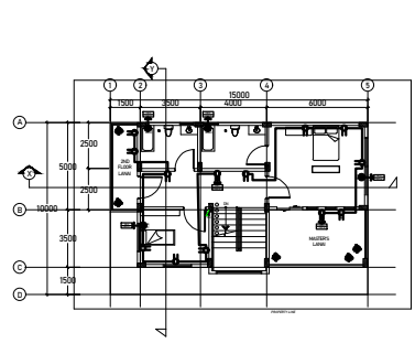
SECOND FLOOR POWER & AUXILIARY LAYOUT SCALE: 1:150
