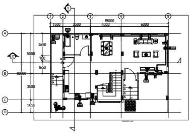
GROUND FLOOR POWER & AUXILIARY LAYOUT SCALE: 1:150
