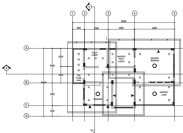
SECOND FLOOR REFLECTED CEILING PLAN SCALE: 1:100
