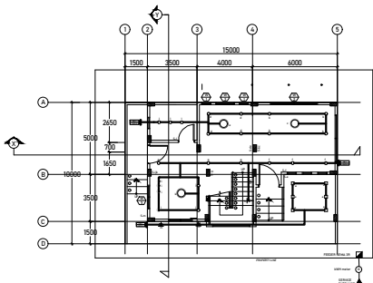
GROUND FLOOR LIGHTING LAYOUT SCALE: 1:150
