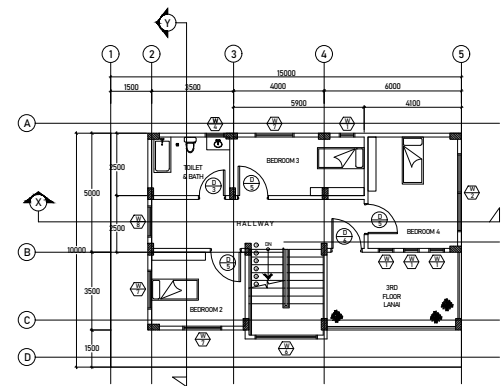
6 A 2 THIRD FLOOR PLAN SCALE: 1:100
