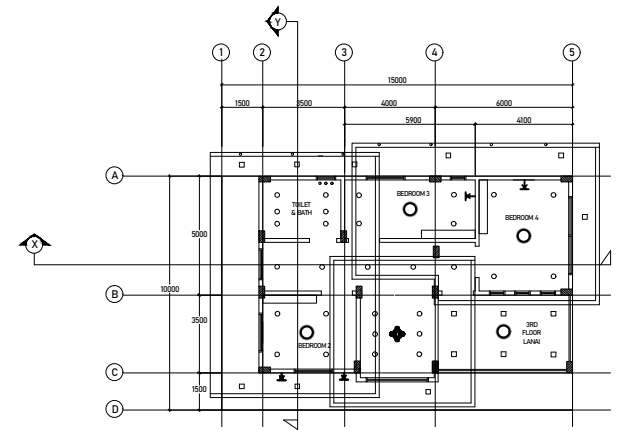
THIRD FLOOR REFLECTED CEILING PLAN SCALE: 1:100
