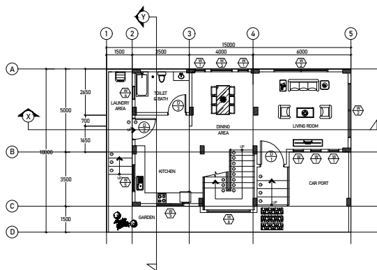
4 A 2 GROUND FLOOR PLAN SCALE: 1:100
