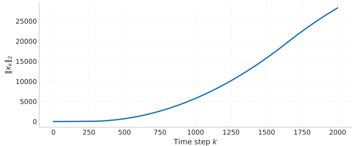
(b) Closed-loop state response
