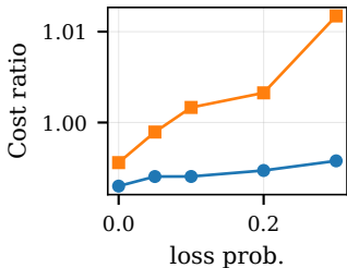
Packet loss
