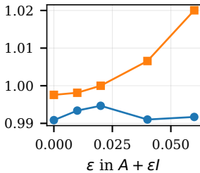
Model mismatch
