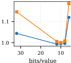
Model mismatch
