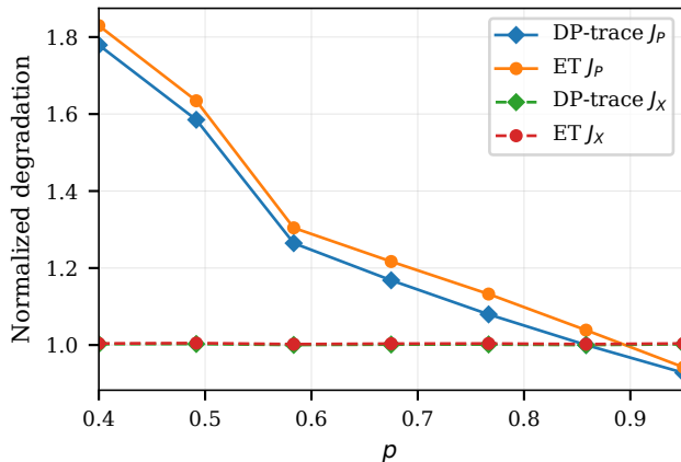
(c) Mismatch degradation vs p
