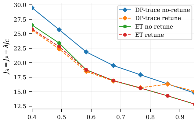
(c) Mismatch degradation vs p
