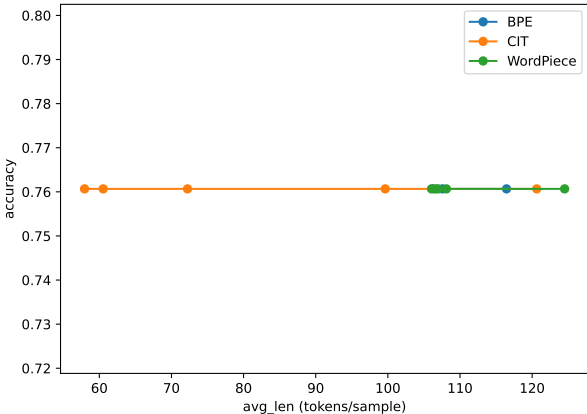
Accuracy vs. Rate (avg token length)
