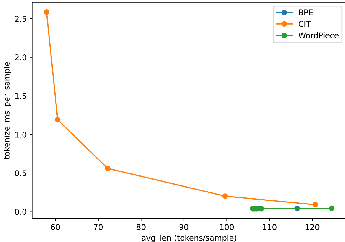
Tokenization Time vs. Rate
