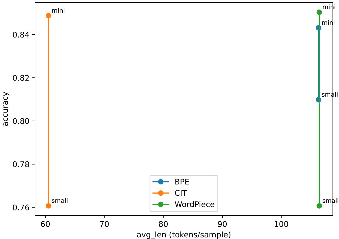
E3 Pareto: Accuracy vs. Rate
