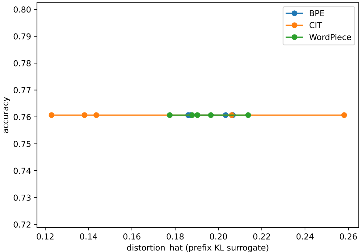
Accuracy vs. Surrogate Distortion
