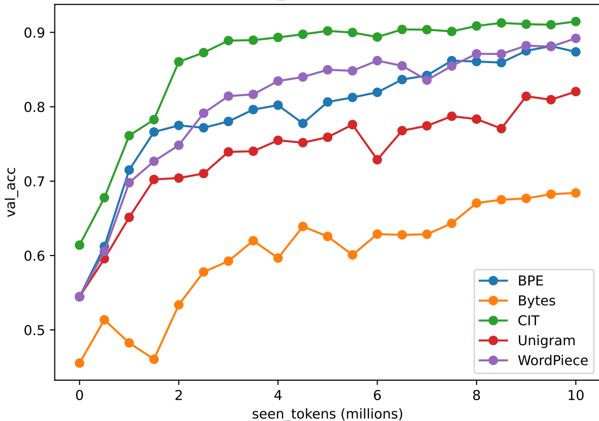
E2 CSIC (token_fair) learning curves (tiny)
