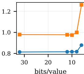
Model mismatch
