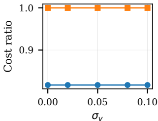
Packet loss
