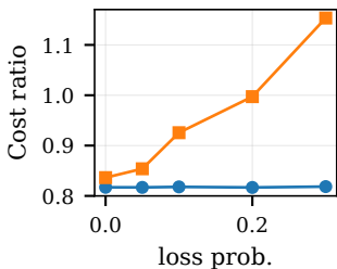
Packet loss
