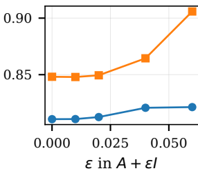
Model mismatch
