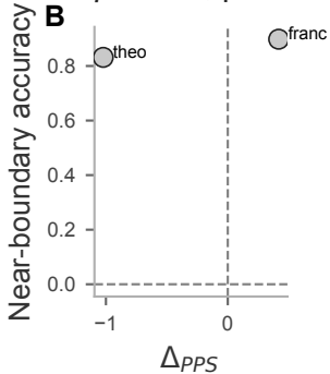
H7a.2 (primary) \rho = \text{nan} , p = \text{nan}
