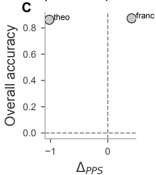
H7a.2 (descriptive) \rho = \text{nan} , p = \text{nan}
