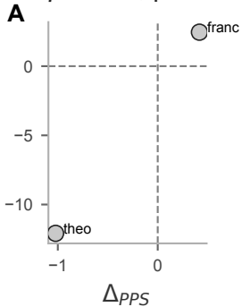
H7a.1 \rho = \text{nan} , p = \text{nan}
