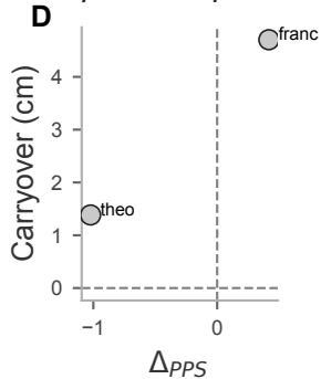
H7a.3 \rho = \text{nan} , p = \text{nan}
