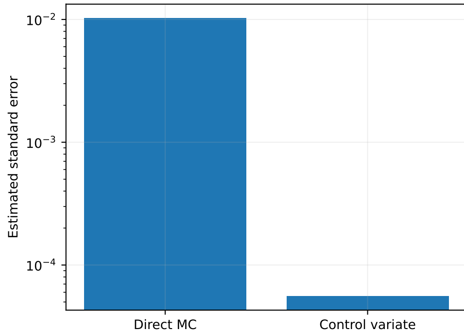
Independent-pilot control variate
