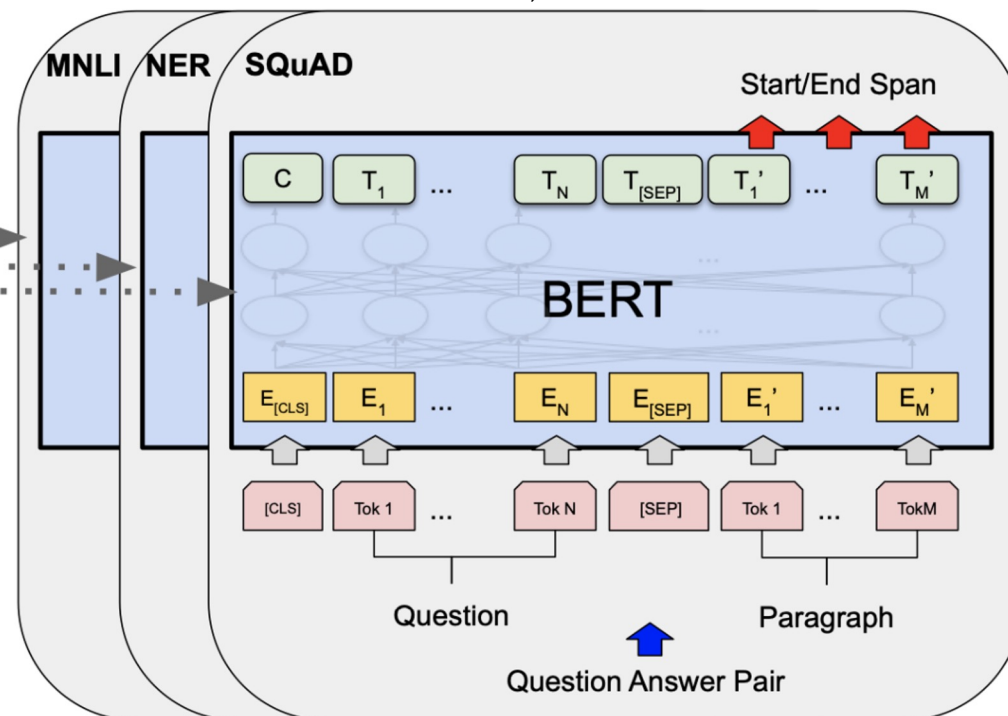
Fine-Tuning
