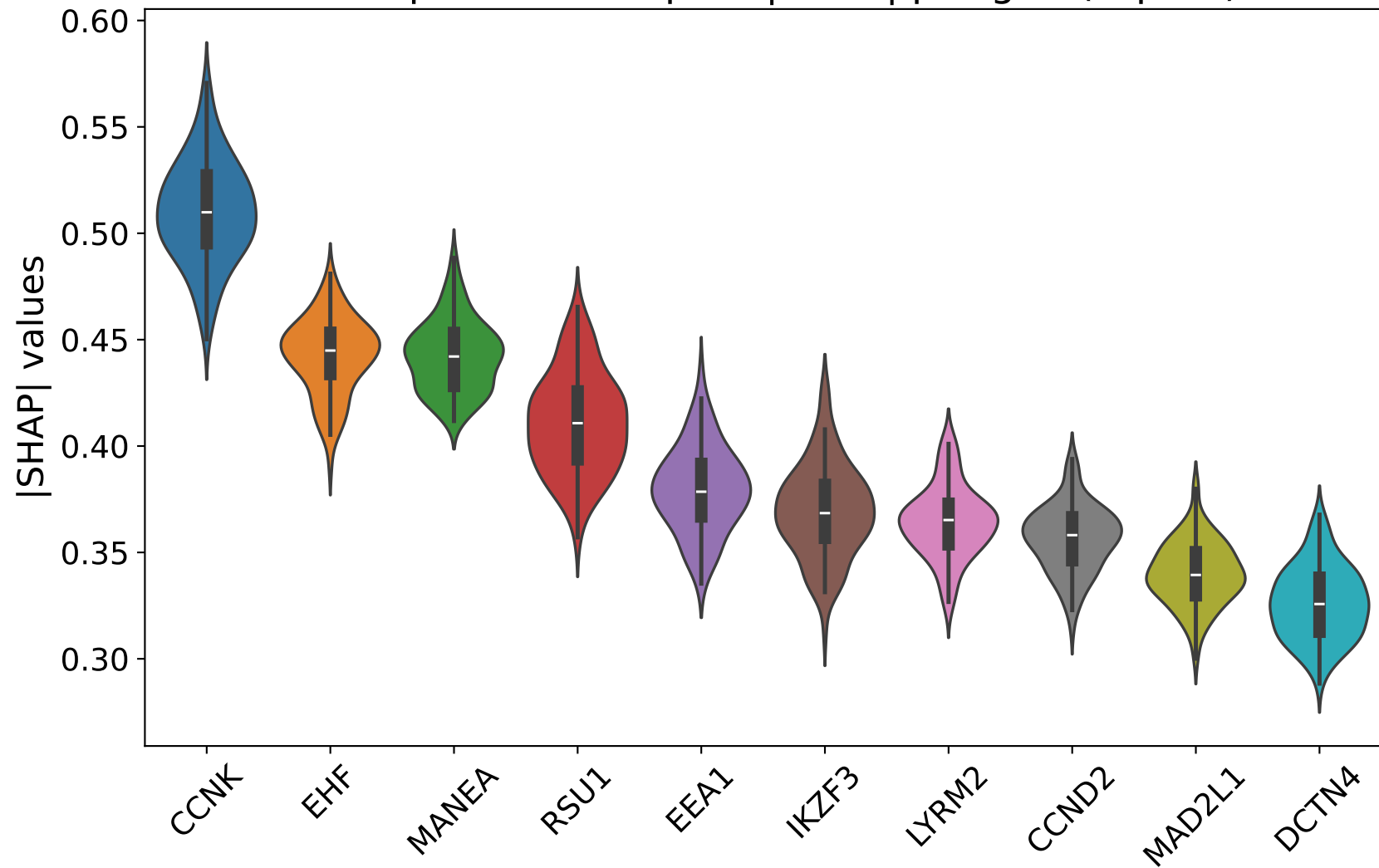
Violin plot bootstrap de |SHAP| por gen (Top 10)
