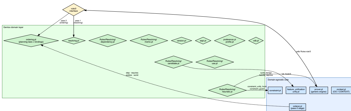
Figure 14 — Layer separation
