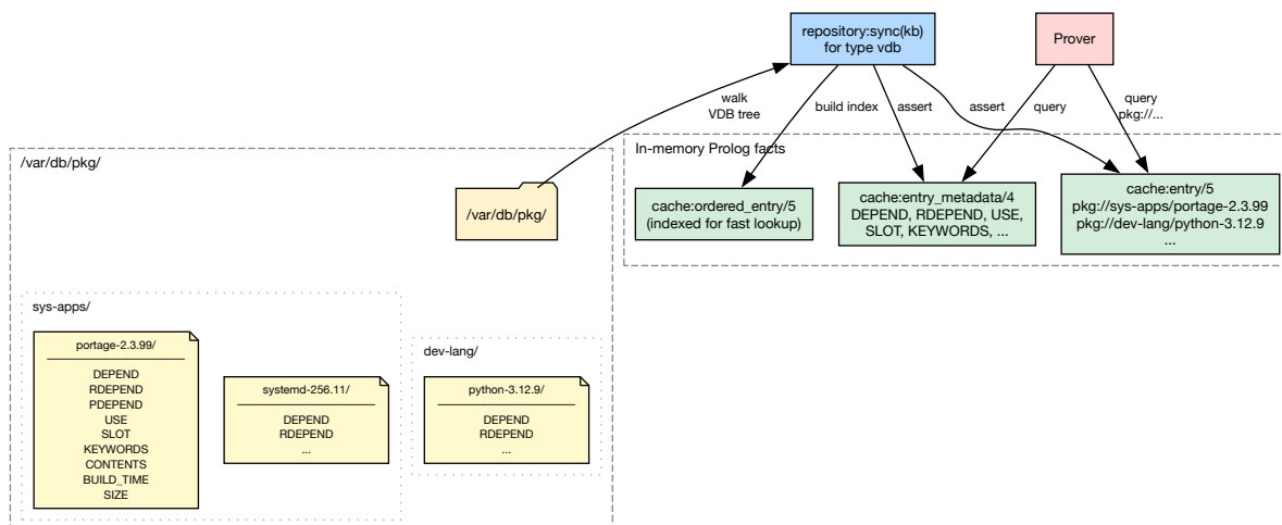
Figure 7 — VDB architecture
