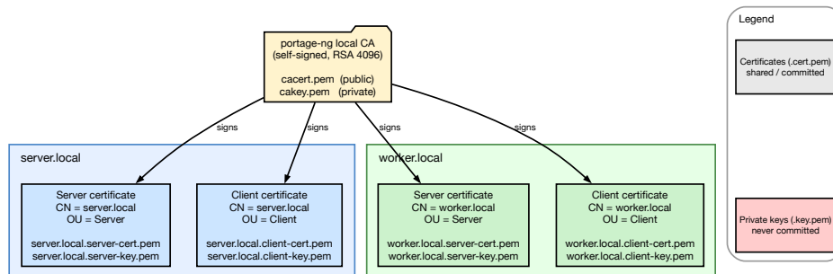
Figure 53 — Certificate hierarchy
