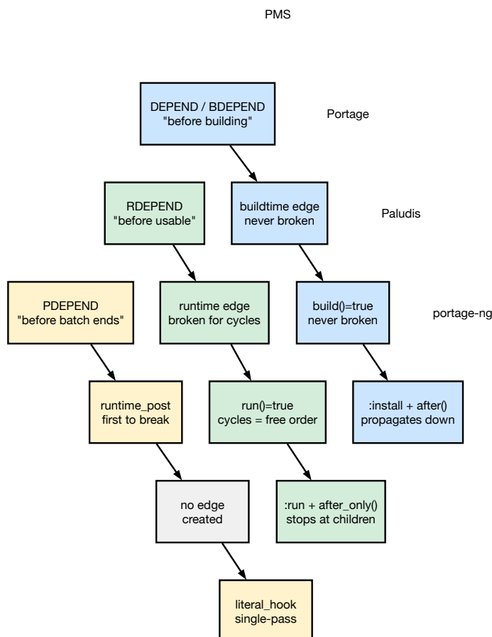
Figure 63 — Dependency type mapping across resolvers
