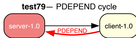
Figure 68 — test79 — PDEPEND cycle
