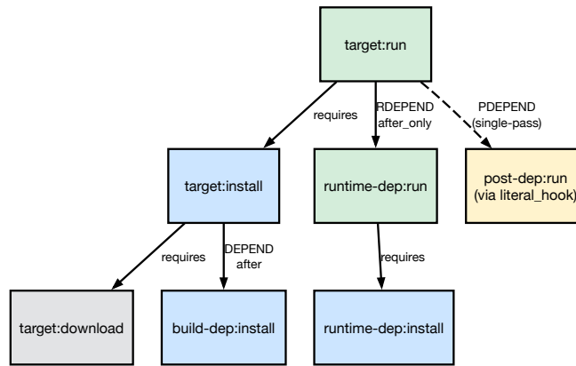
Figure 62 — portage-ng two-phase dependency model
