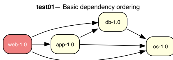
Figure 64 — test01 — Basic dependency ordering
