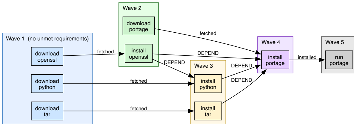
Figure 38 — Wave plan produced by the ordering pass
