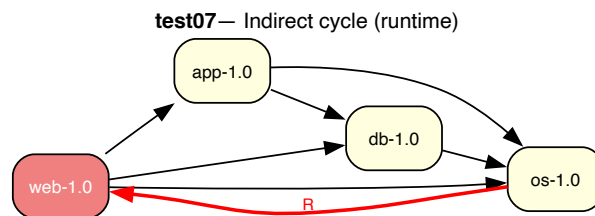
Figure 66 — test07 — Indirect cycle (runtime)
