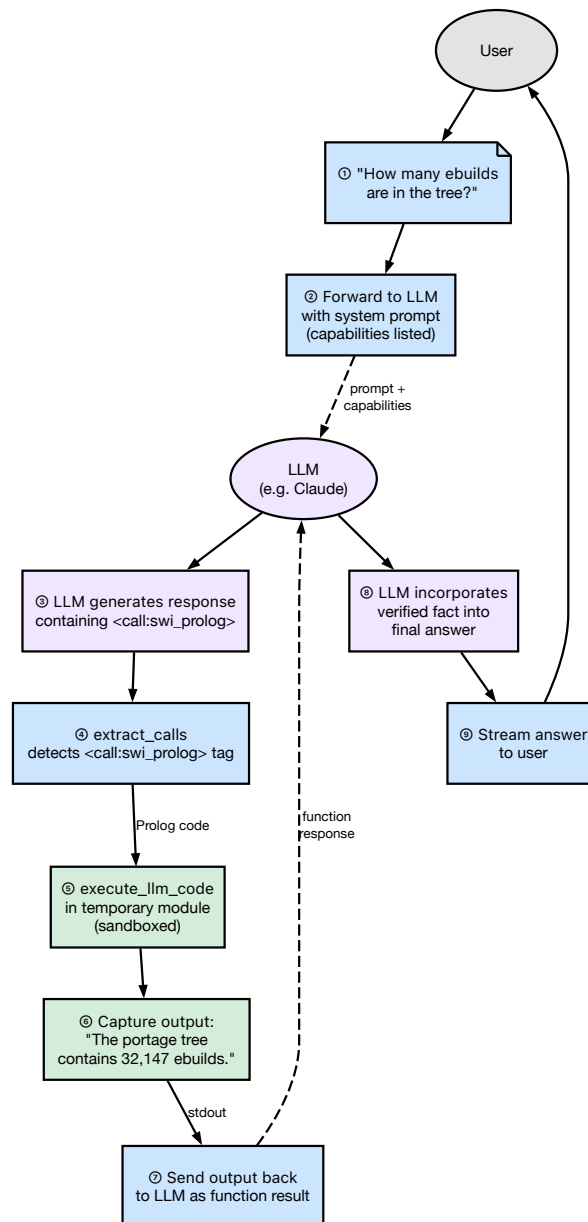
Figure 43 — Code execution round trip
