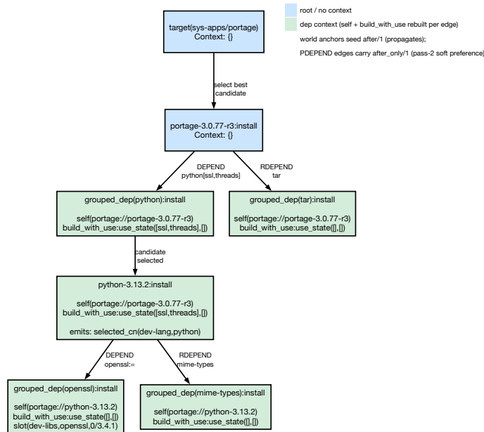
Figure 56 — Context evolution through a dependency chain
