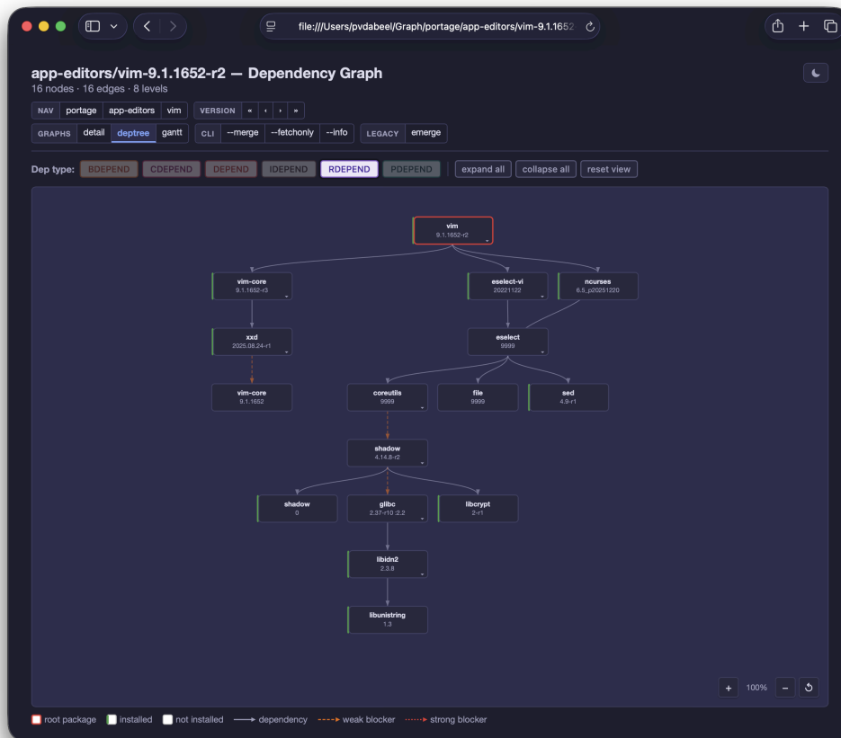
Figure 39 — Dependency graph for app-editors/vim
