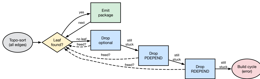
Figure 61 — Portage progressive edge relaxation
