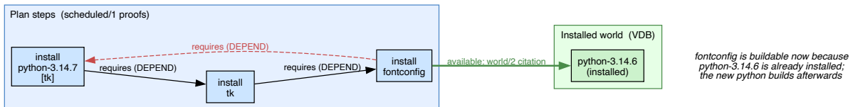
Figure 37 — Ordering a cycle through the installed world
