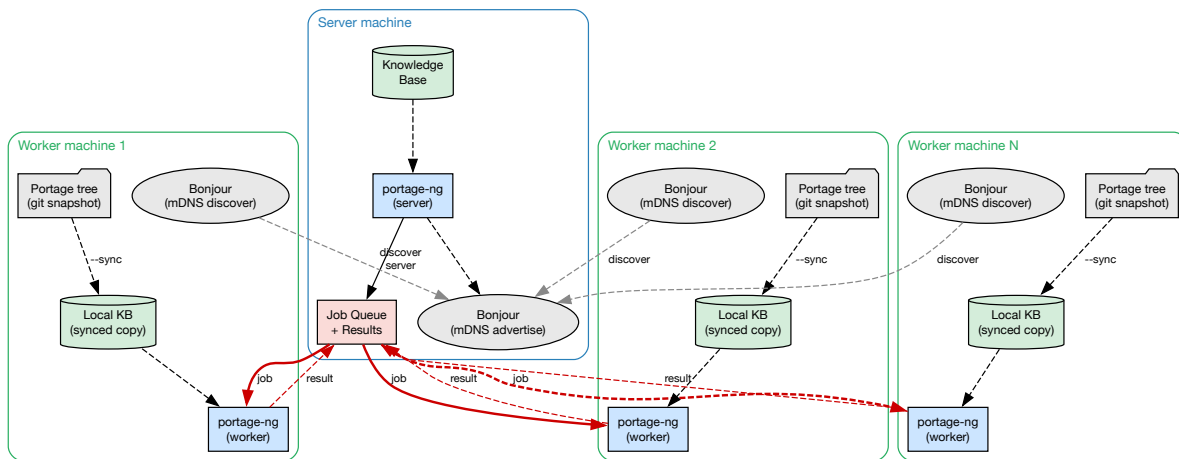
Figure 11 — Worker mode
