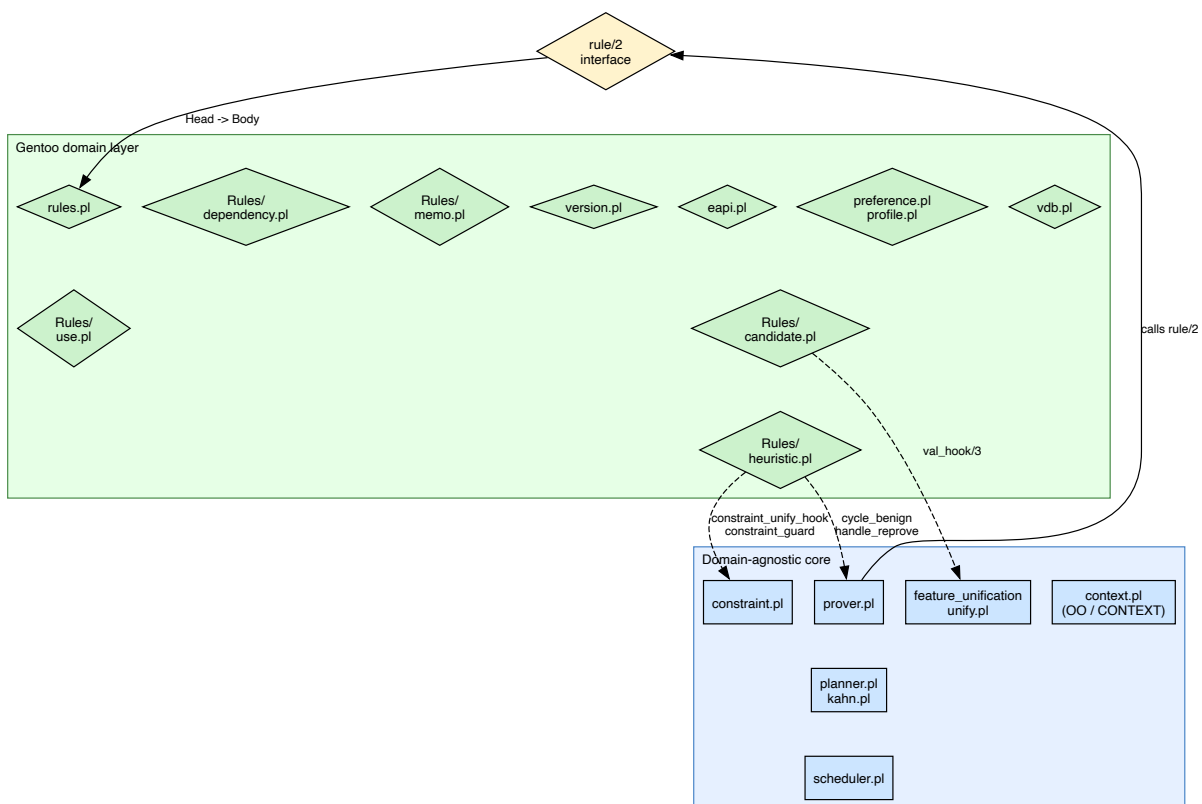
Figure 12 — Layer separation
