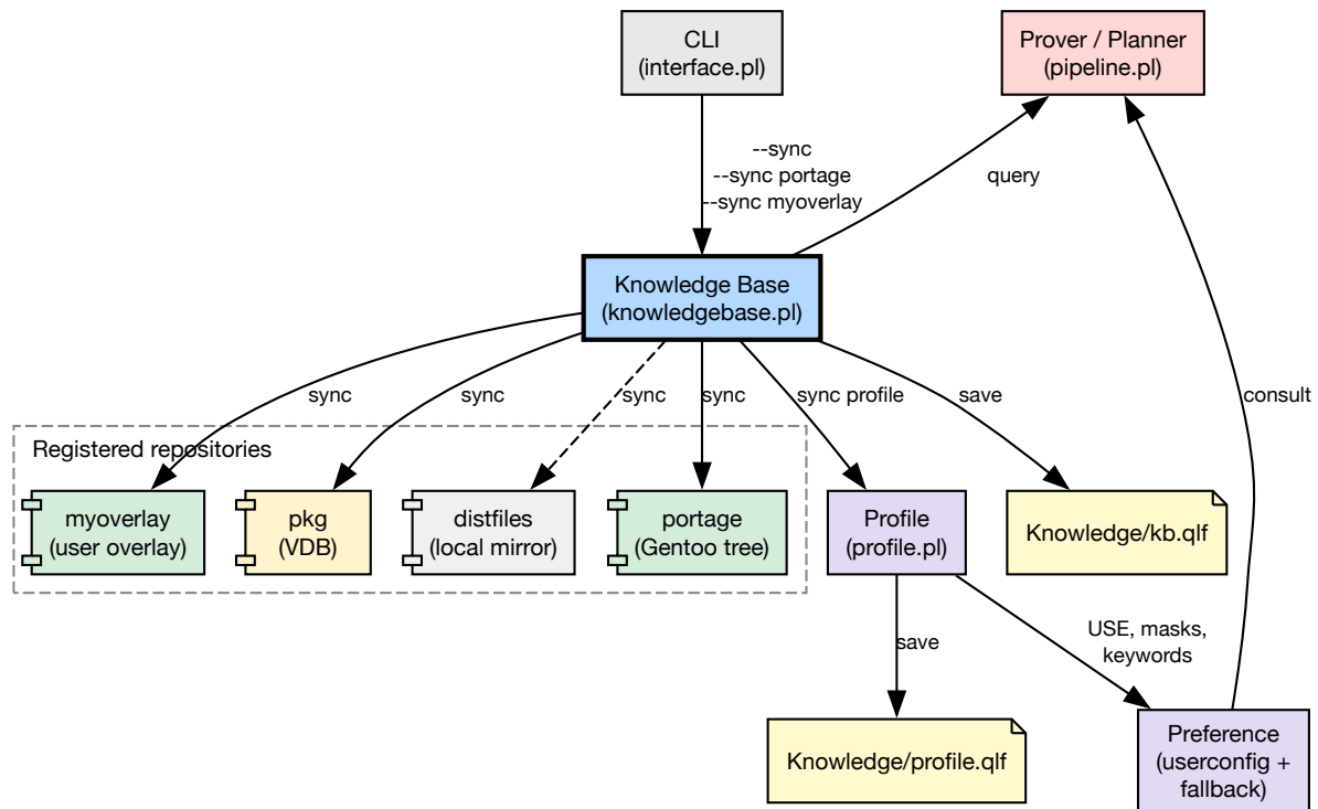
Figure 4 — Sync architecture
