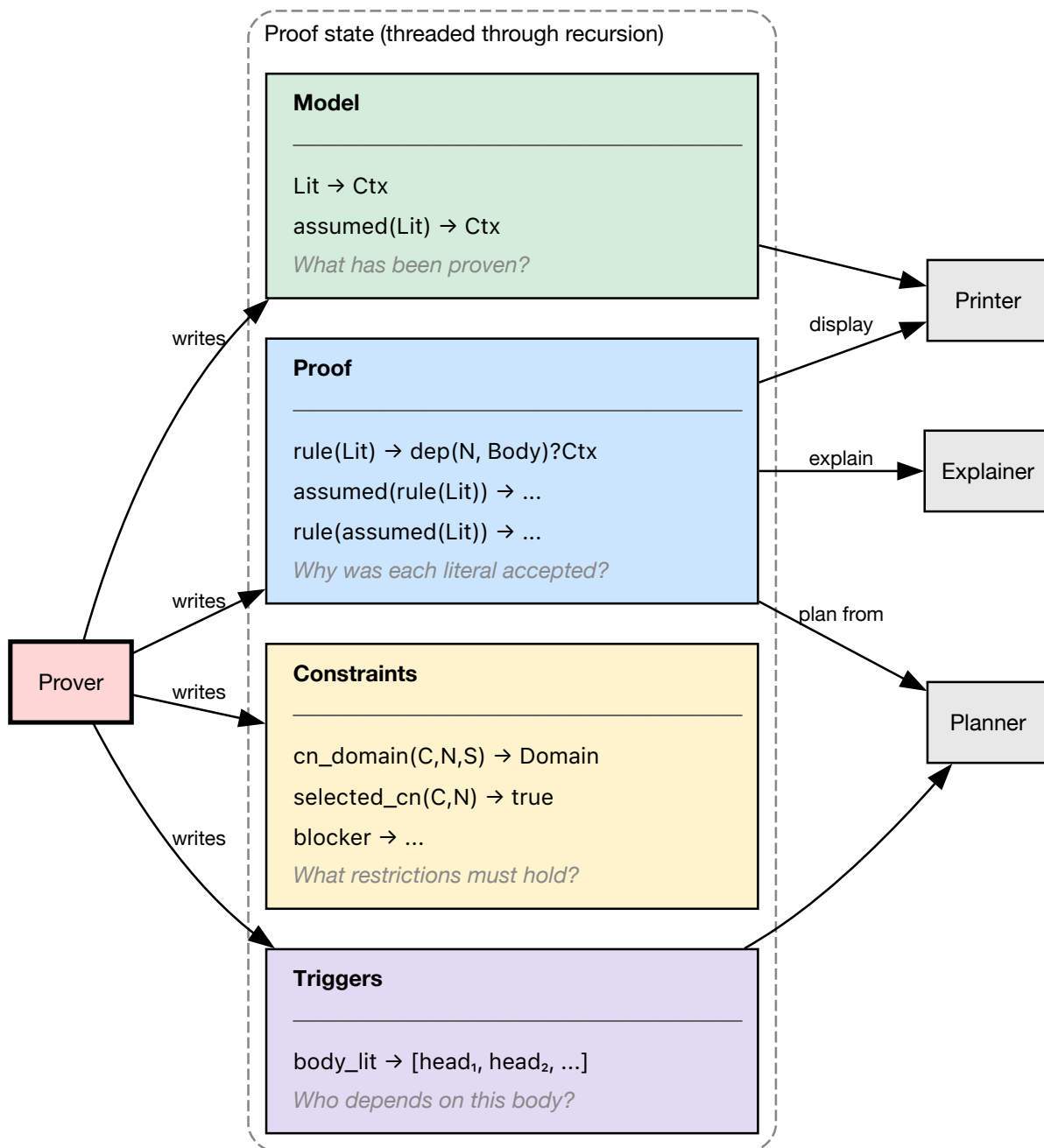
Figure 13 — Data structures
