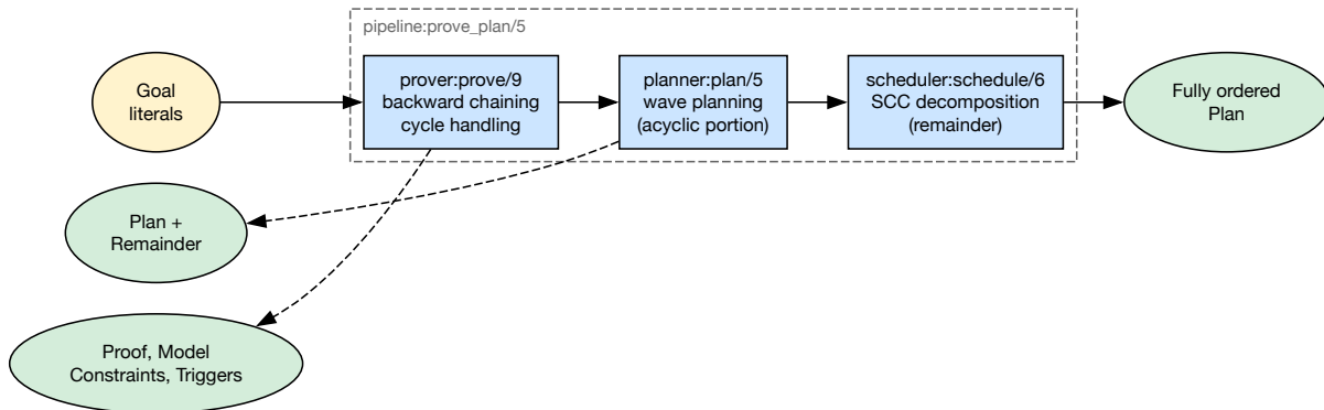
Figure 21 — prove_plan pipeline
