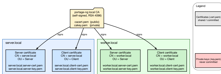
Figure 47 — Certificate hierarchy
