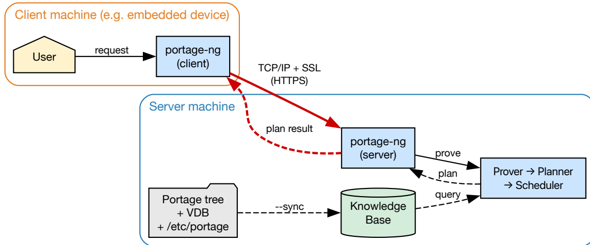
Figure 9 — Client–server mode
