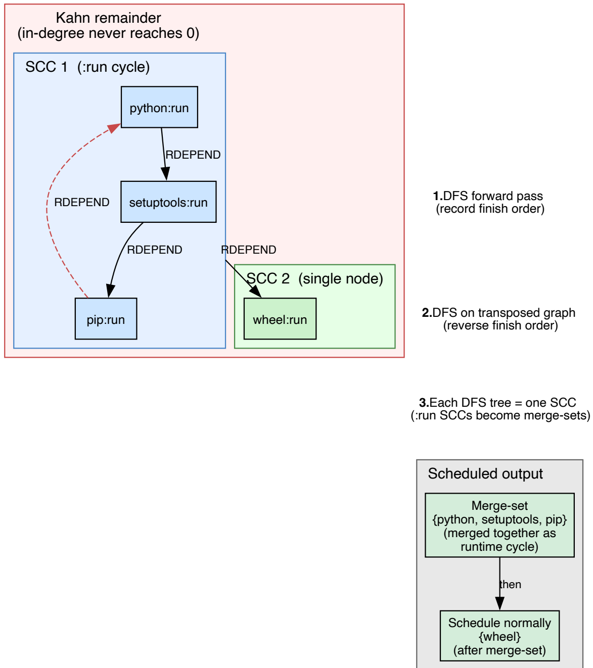
Figure 36 — SCC scheduling example
