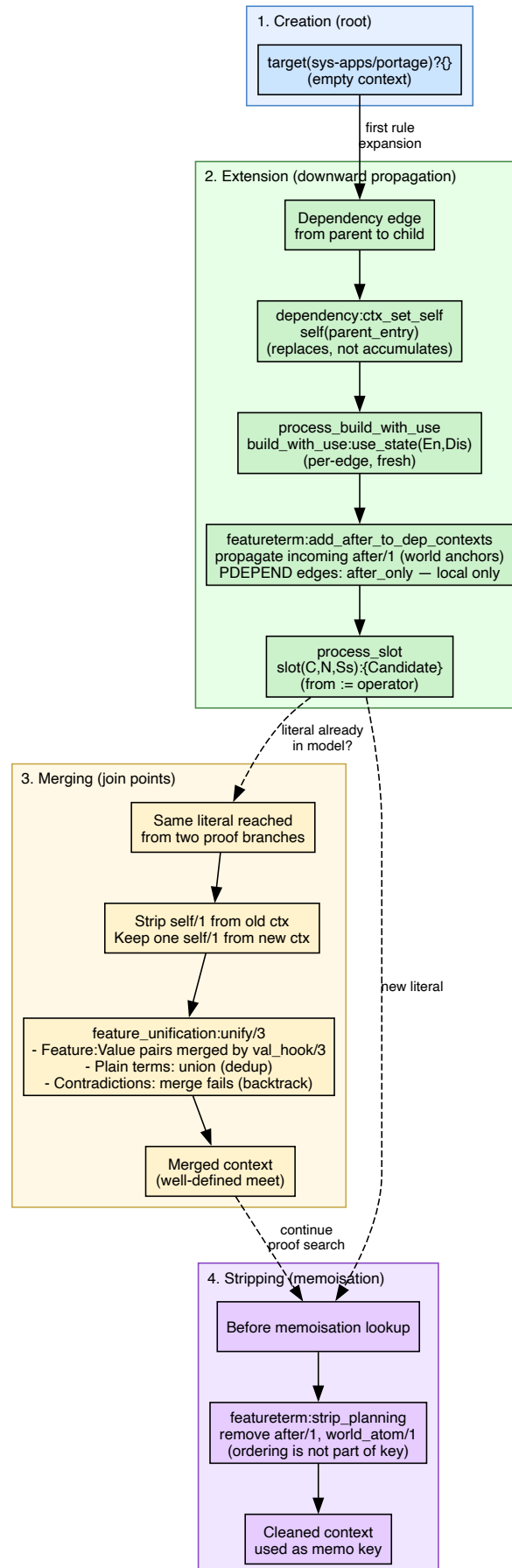
Figure 52 — Context lifecycle
