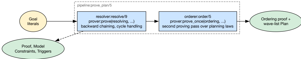
Figure 21 — prove_plan pipeline
