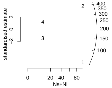
Figure 10: Radial plot for the toy example of Table 1, with \zeta = 350 yr \text{cm}^2 and \rho_D = 2.5 \times 10^6 \text{ cm}^{-2} . Connecting the origin of the diagram to the plot symbols for grains 1 and 3 (low N_s/N_i -ratios) forms a line with a negative slope, which projects onto the radial scale at a younger date than a line connecting the origin to grains 2 and 4 (high N_s/N_i -ratios, positive slope). Grains 1 and 2 (high N_s + N_i -values, right hand side of the radial plot) are more precise than grains 3 and 4 (low N_s + N_i -values, left hand side of the radial plot).
