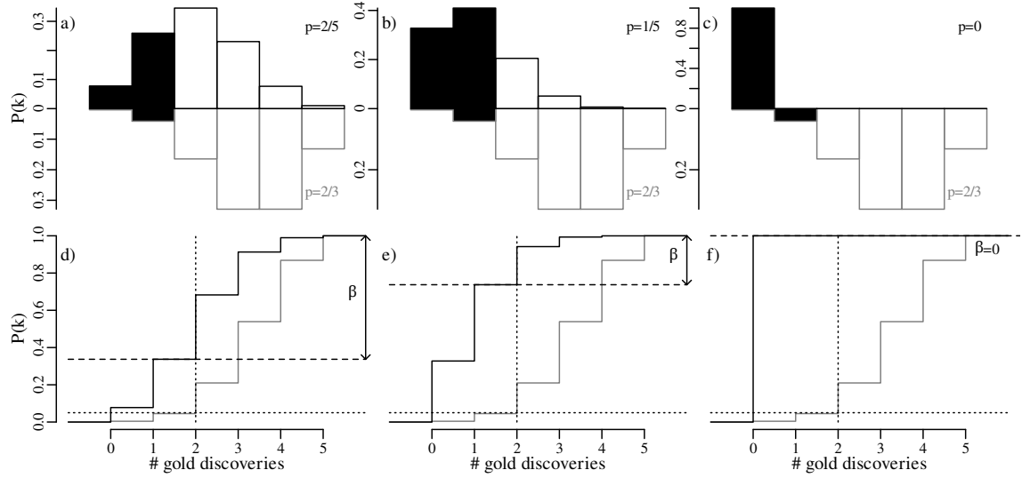
Figure 5.8: a) – c) PMFs of the binomial null distribution with p = 2/3 ( H_0 , black and grey, bottom) and alternative distributions ( H_A , black and white, top) with a) p = 2/5 , b) p = 1/5 and c) p = 0 . Sample size is n = 5 for all cases. d) – f) CDFs for the null distribution (grey) and the alternative distribution (black). The horizontal dotted lines mark \alpha = 0.05 . Their intersections with the CDF of the null distribution are marked by vertical dotted lines. The areas to the left of these lines define the rejection region under a one-sided test and are marked in black in the PMFs of the alternative distributions (a – c). The dashed horizontal lines mark the intersection of the rejection boundary with the CDF of the alternative distribution. They mark the power of the statistical test ( 1 - \beta ). Power increases as the alternative distribution drifts away from the null distribution.
