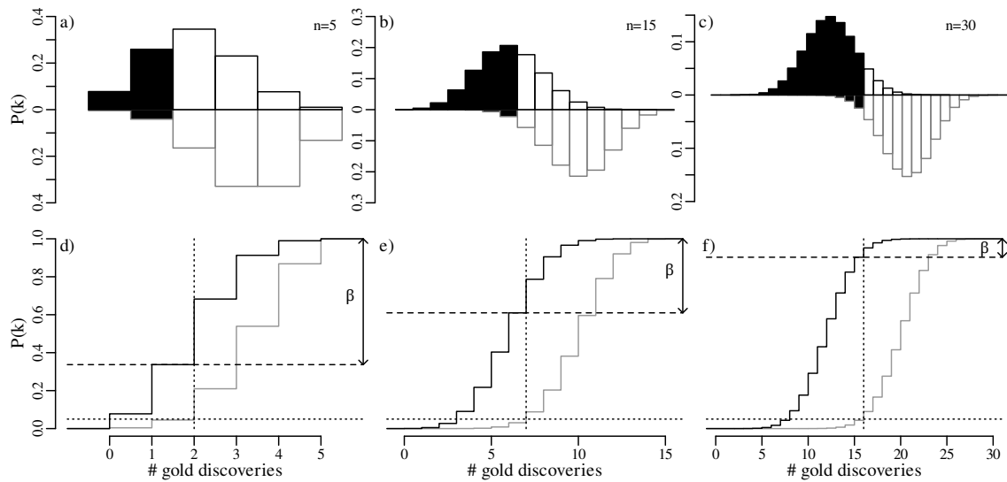
Figure 5.9: a) – c) PMFs of binomial distributions with p = 2/3 ( H_0 , black and grey, bottom) and p = 2/5 ( H_A , black and white, top), for sample sizes of a) n = 5 , b) n = 15 and c) n = 30 . d) – f) CDFs for the null distribution (grey) and the alternative distribution (black). The horizontal dotted lines mark \alpha = 0.05 , corresponding to a one-sided test. Their intersections with the CDF of the null distribution are marked by vertical dotted lines. The area to the left of these lines define the rejection region and are marked in black in the bar chart. The larger the sample size, the easier it is to reject H_0 . The dashed horizontal lines mark the intersection of the rejection region with the CDF of the alternative distribution. These mark the power of the statistical test ( 1 - \beta ). Power increases with sample size.
